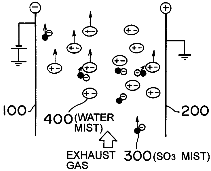
FIG.24 (RELATED ART)
