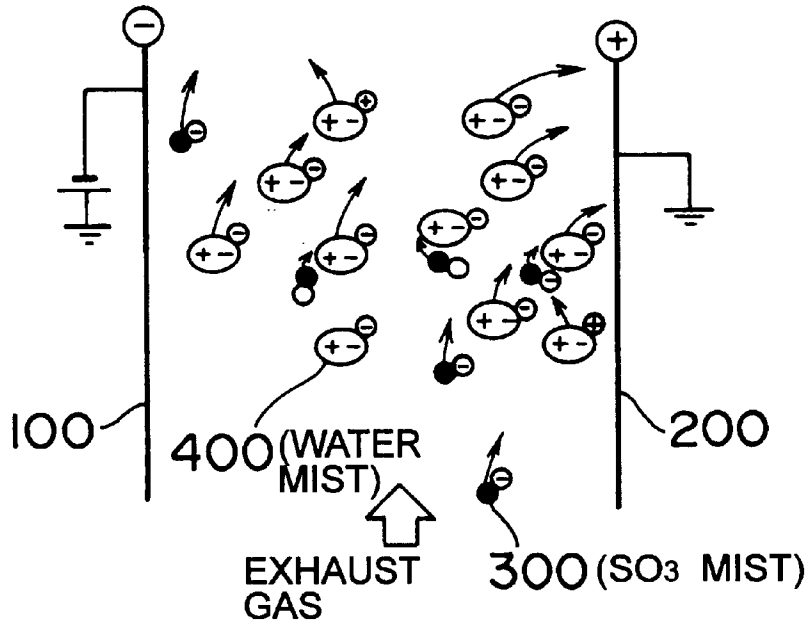
FIG.26 (RELATED ART)
