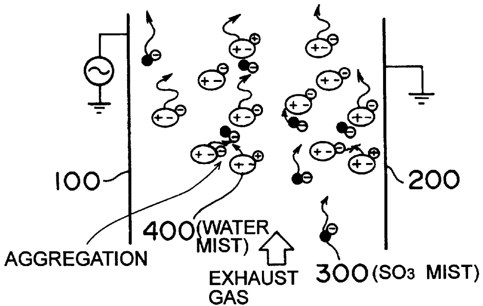
FIG.27 (RELATED ART)
