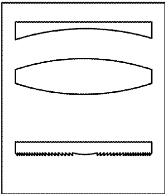
COMBINATION OF FRESNEL LENSES AND REFRACTIVE LENSES
