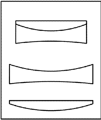
COMBINATION OF REFRACTIVE LENSES WITH NONZERO DISPERSION
