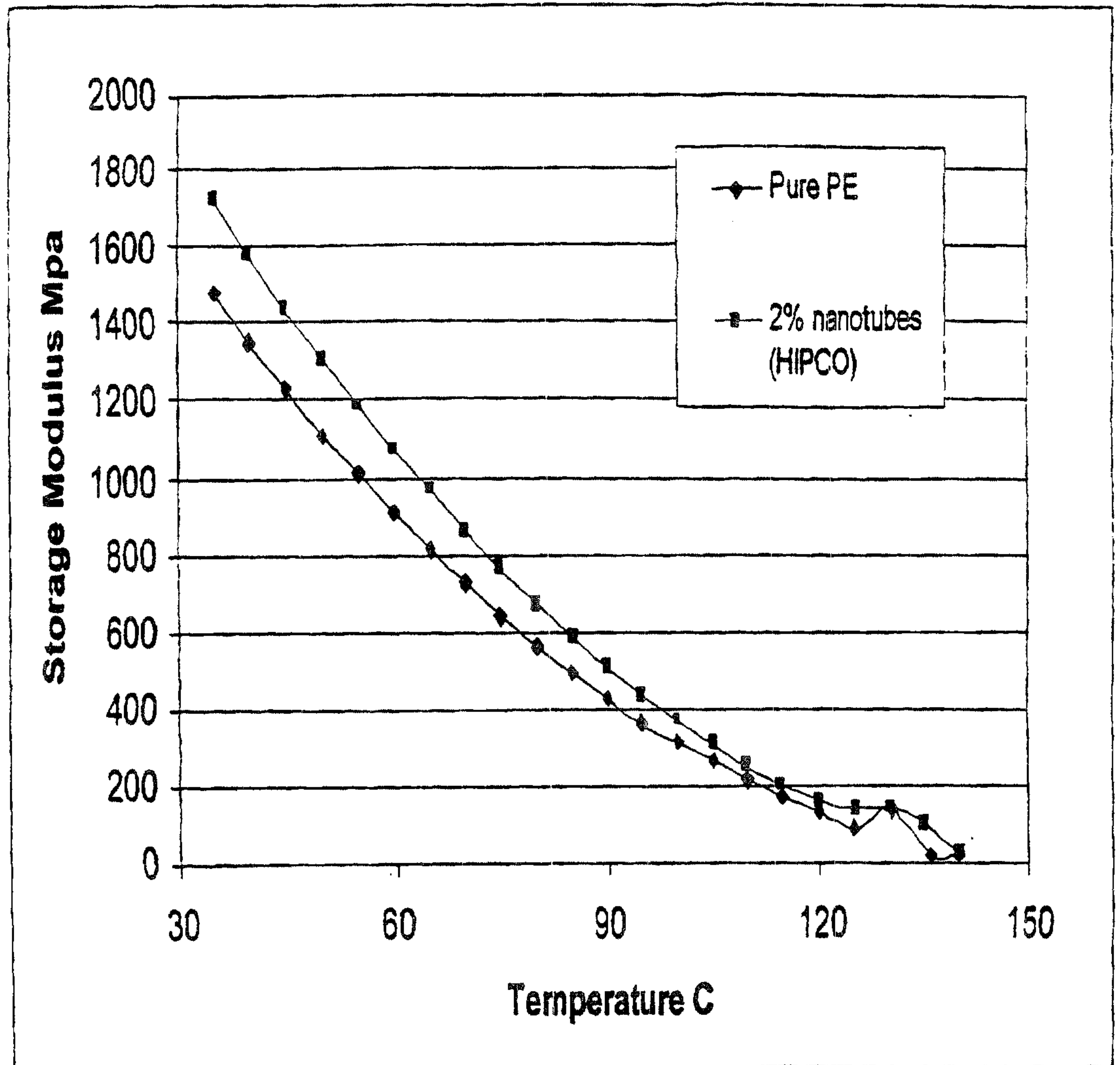
Figure 12 Storage modulus vs. temperature. For PE with and without SWNTs
