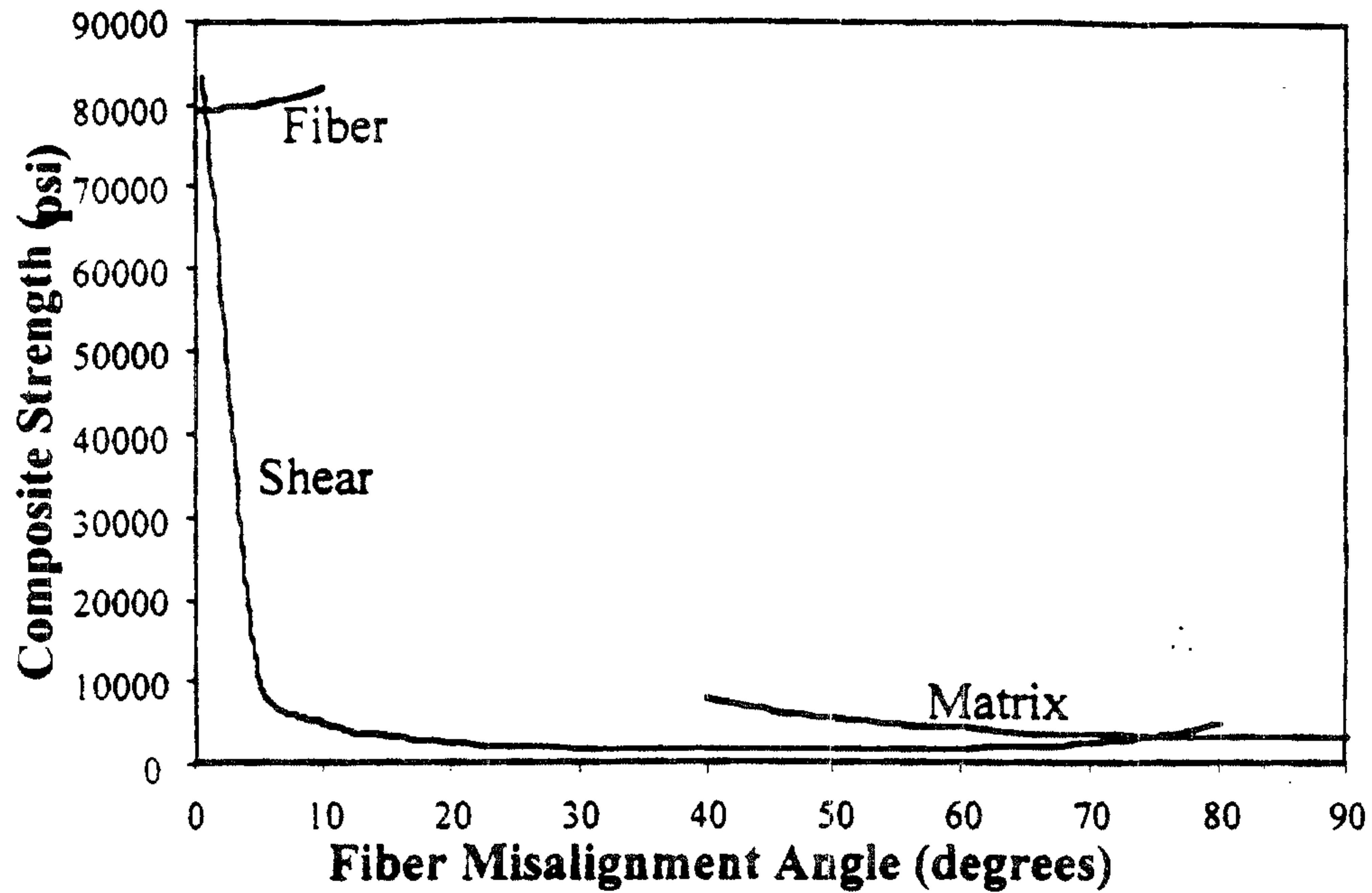
Figure 29 Composite strength vs. the orientation of the SWNTs when considered to be fully aligned. Note that initially when all fibers are aligned with the applied load the strength of the composite is rather high. As the fibers become misoriented with the load (as in the case of an isotropic composite where SWNTs are randomly dispersed), the composite strength goes way down due to low shear and normal strength contributions. On one hand you might use conventional processing to improve the shear and normal stresses where as we take the approach to fully integrate and therefore remove defects that might also result in the matrix.
