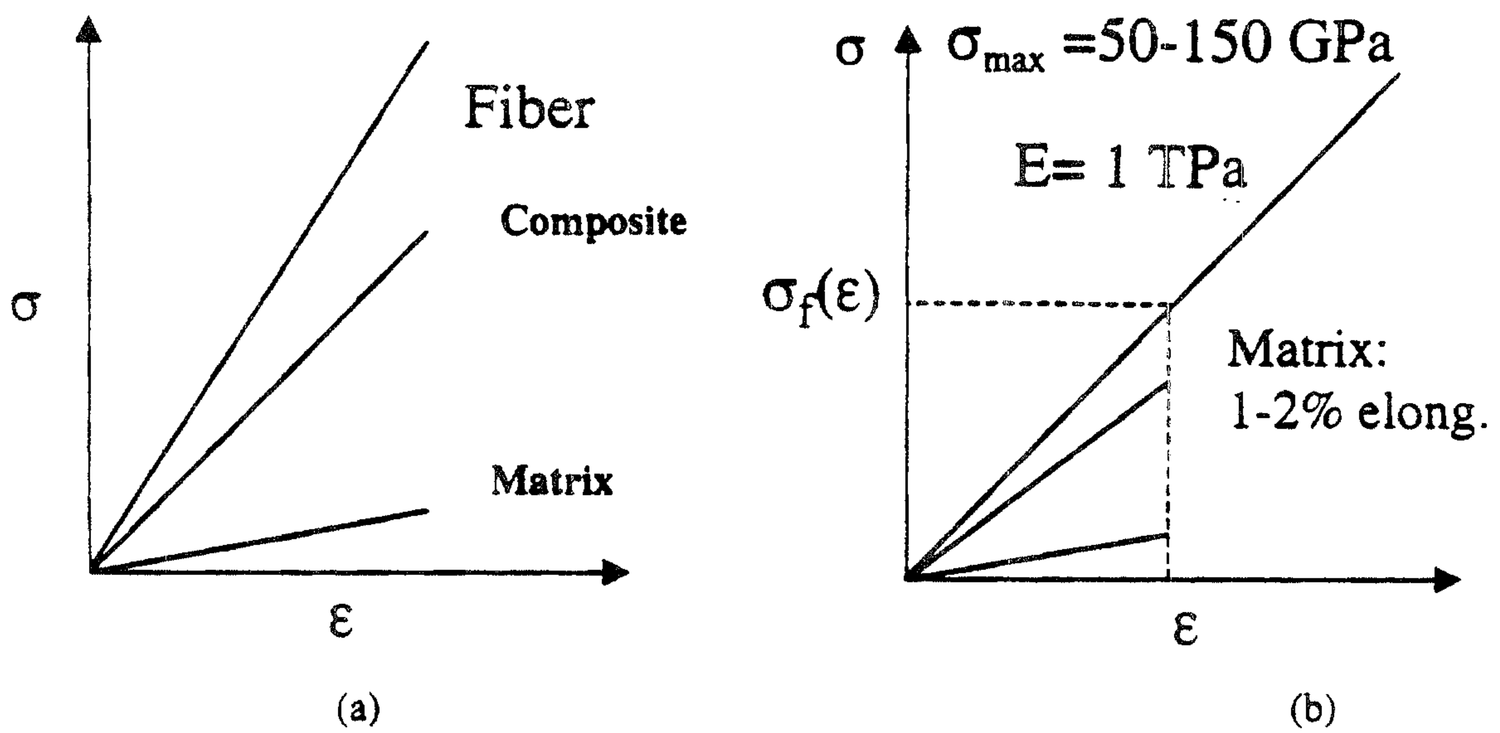
Figure 45 Comparison of a stress-strain curve for (a) a typical epoxy composite compared to that for (b) a nanotube composite where significant strength of the nanotube is discarded. SWNTs are expected to have a high degree of elongation to failure.
