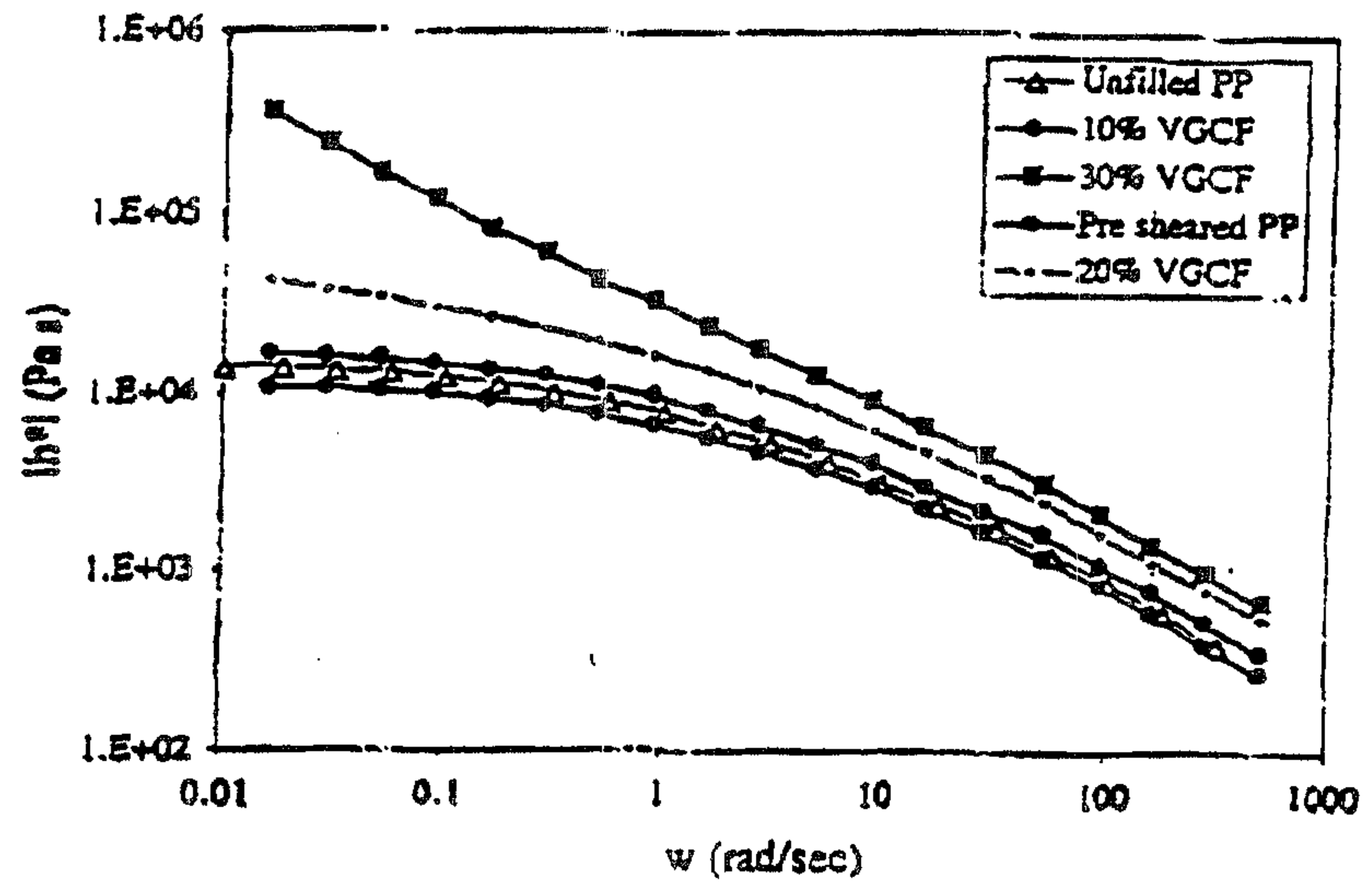
Figure 5. Viscosity vs. shear rate
