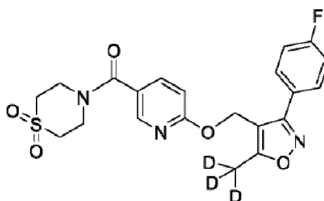
Formel II.
