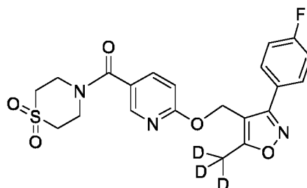
Formula II.
