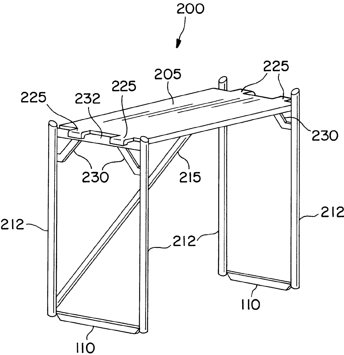
FIG. 9 PRIOR ART
