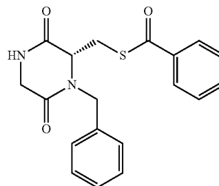
Synthesis of (6R)-6-[(benzoylsulfanyl)methyl]-1-benzylpiperazine-2,5-dione (Pro-4011)
