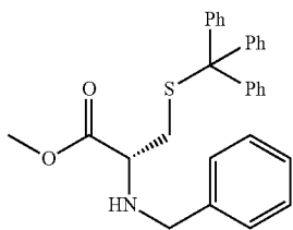
(2R)-2-Benzylamino-3-tritylsulfanyl-propionic acid methyl ester
