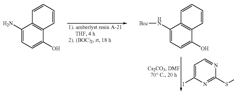
Scheme 3
