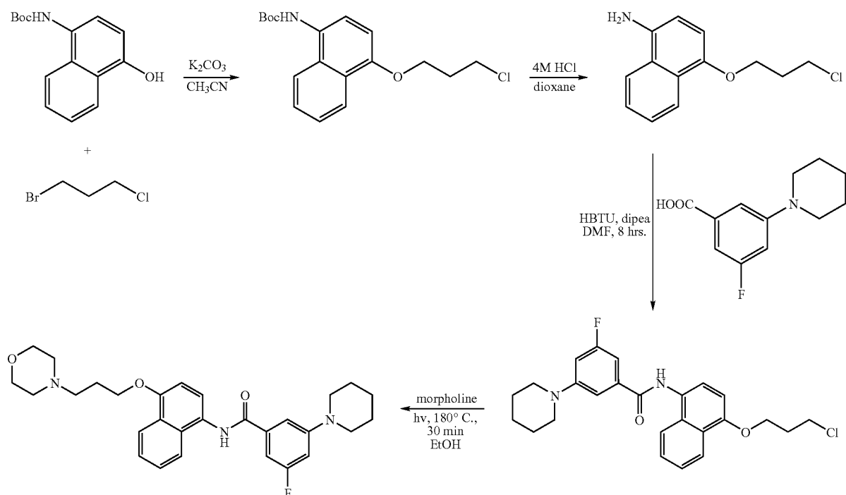
Scheme 7
