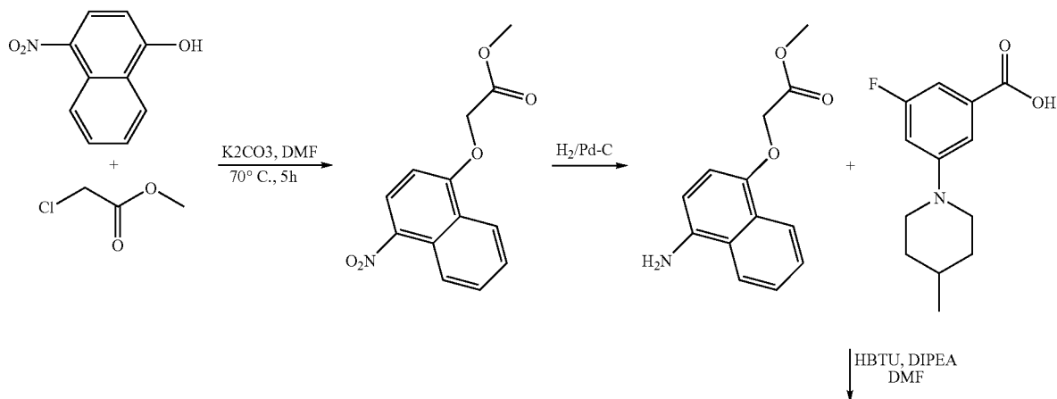
Scheme 10
