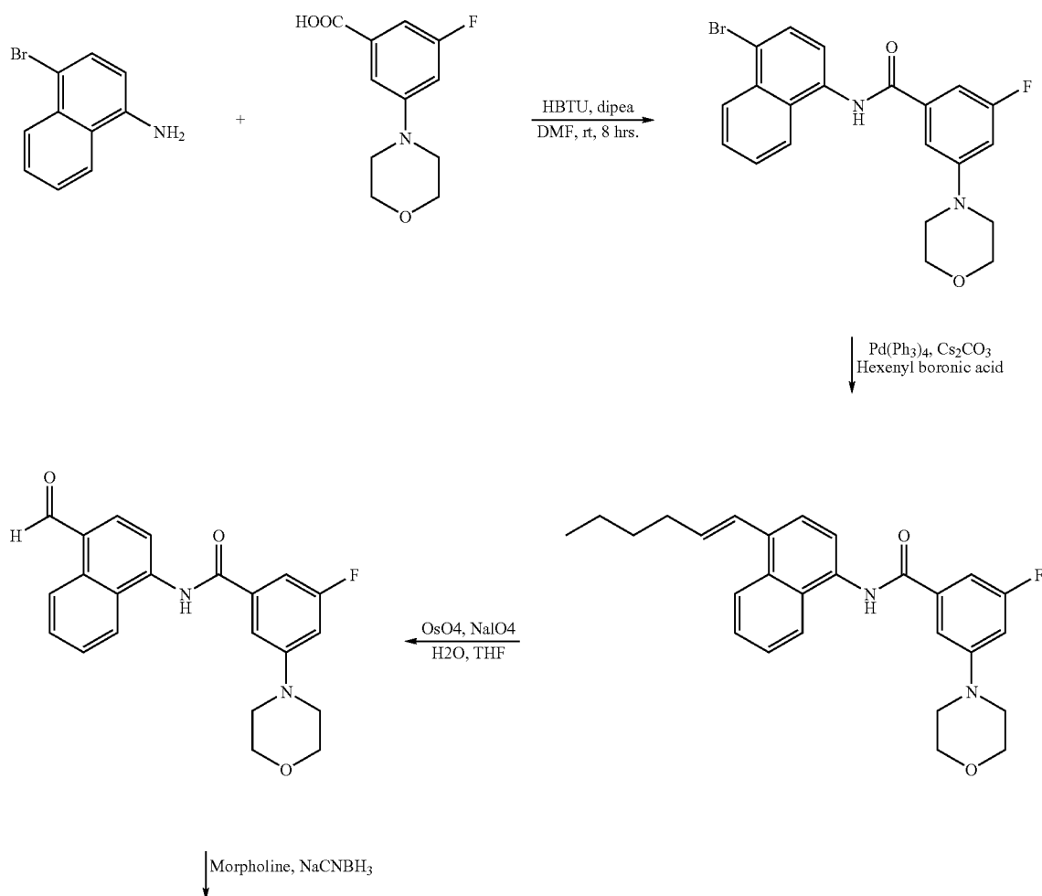
Scheme 15
