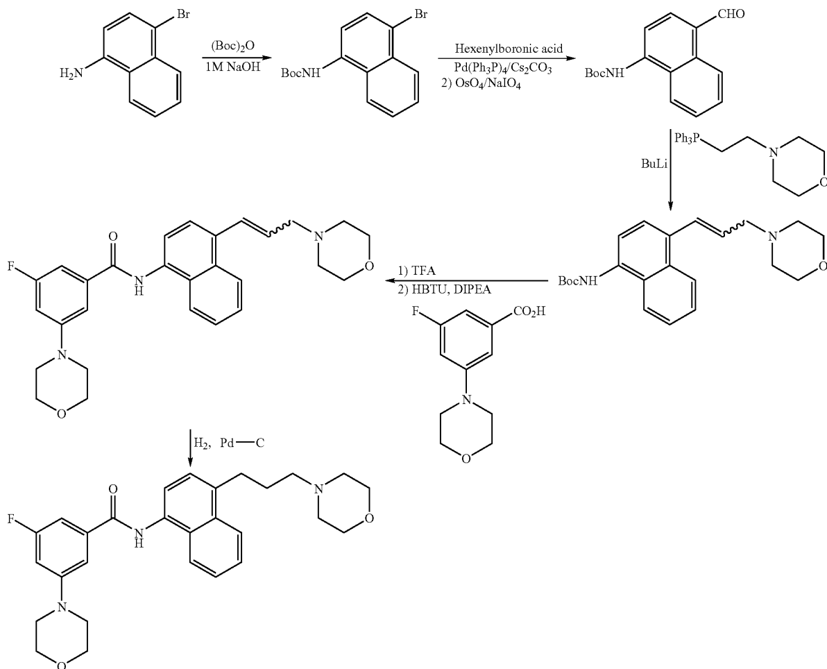
Scheme 11
