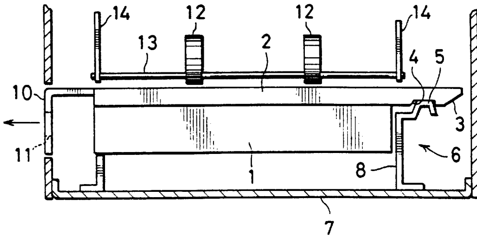
PRIOR ART FIG. 9
