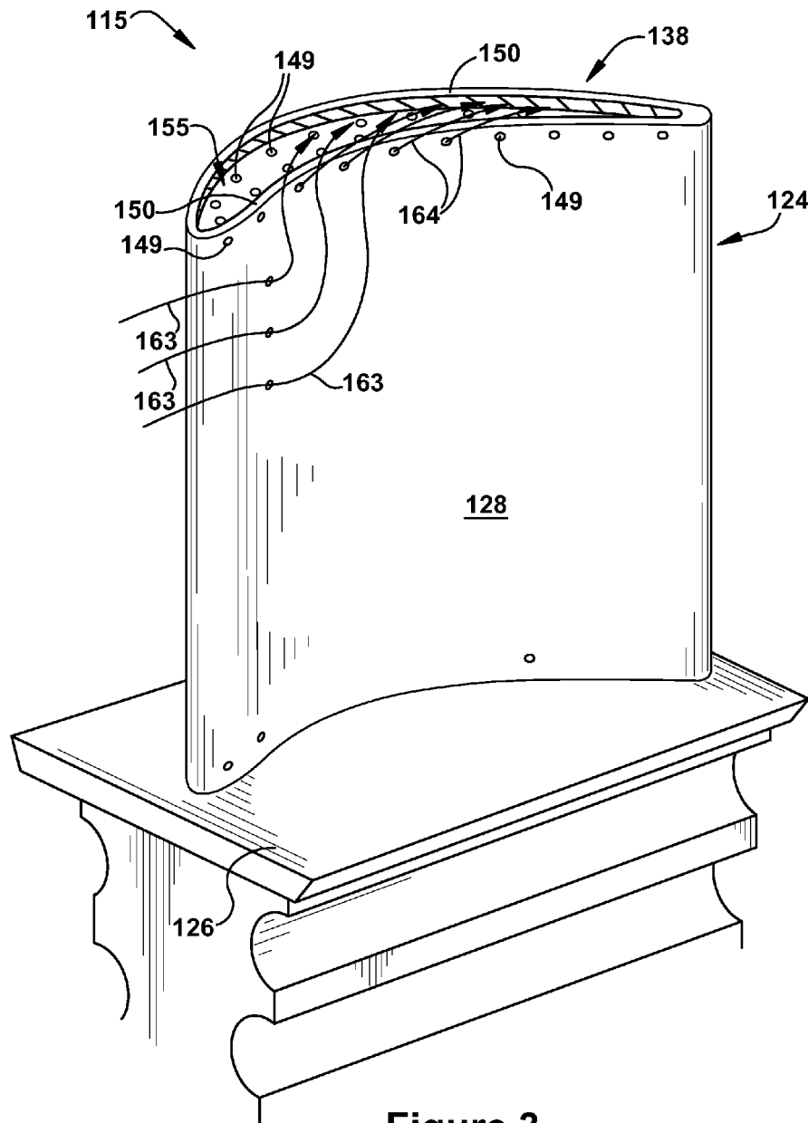
Figure 3 (Prior Art)
