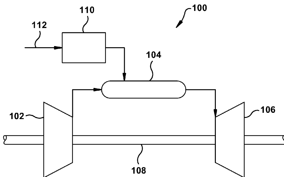
Figure 1 (Prior Art)
