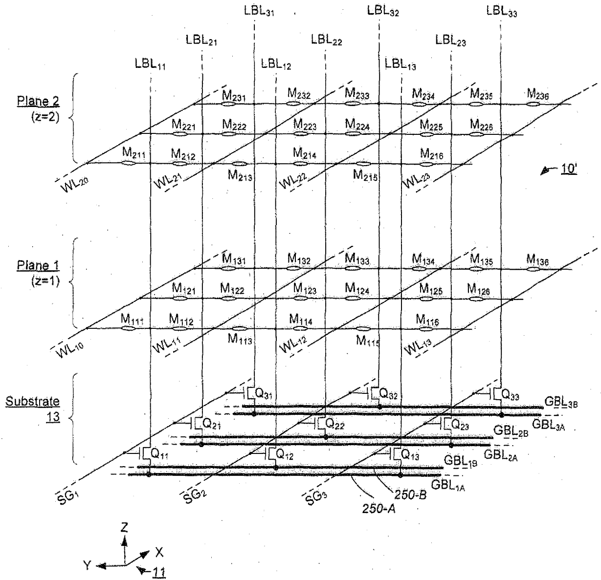
Double-Global-Bit-line Structure
