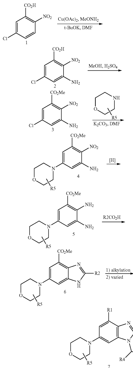
Scheme VII
