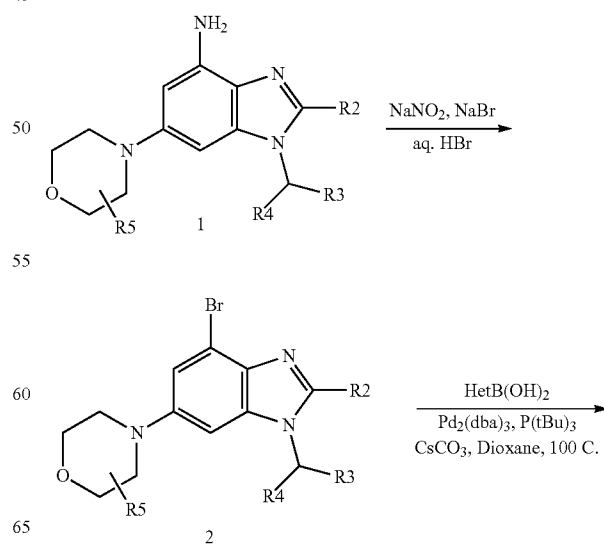
Scheme IV
