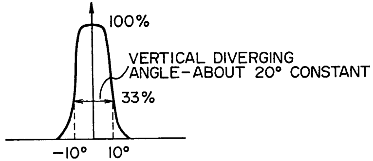
FIG. 9 PRIOR ART
