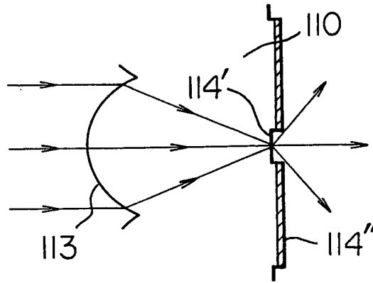
FIG. 7 PRIOR ART
