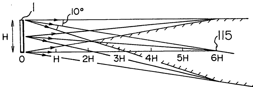
FIG. 10 PRIOR ART
