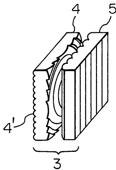
FIG. 2 PRIOR ART
