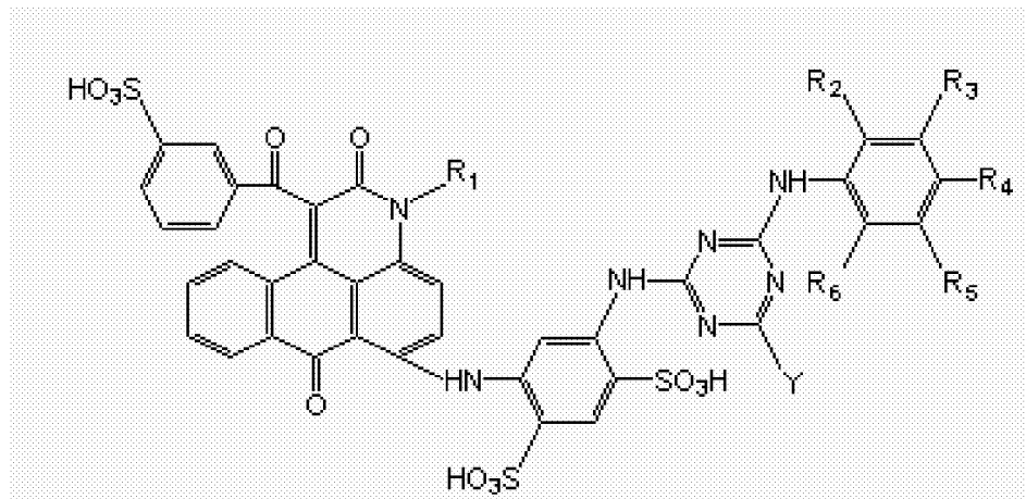
General formula (I)
