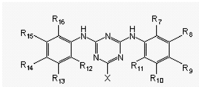
General formula (II)
