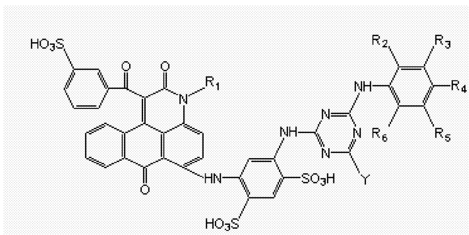
General formula (I)
