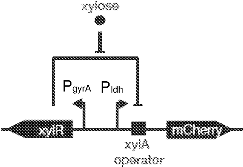
XylR-mCherry- P_{ldh}+XylA
