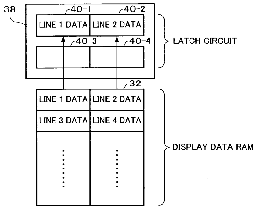
FIG. 4A FIRST READ OPERATION
