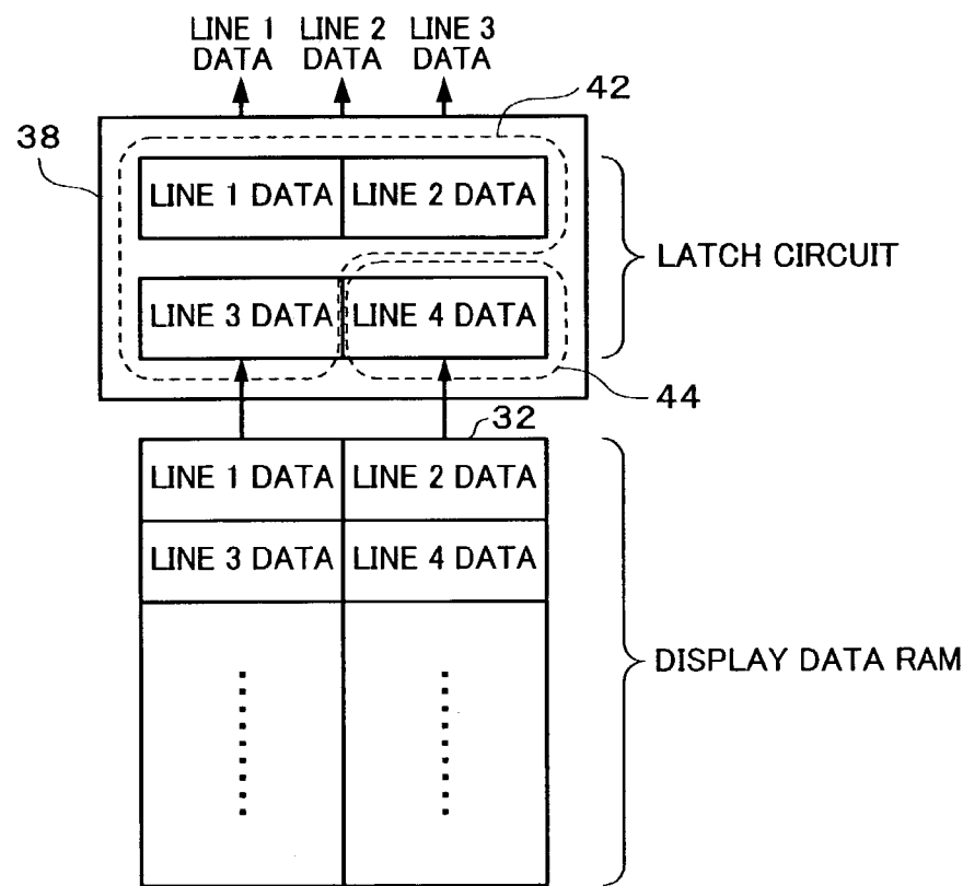
FIG. 4B SECOND READ OPERATION
