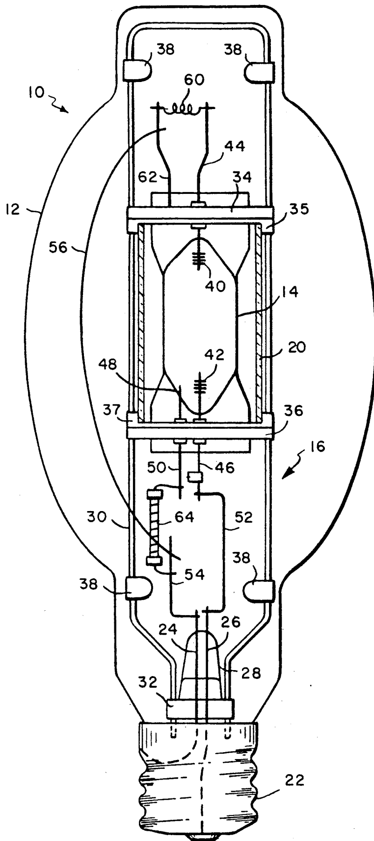
FIG. 1 PRIOR ART
