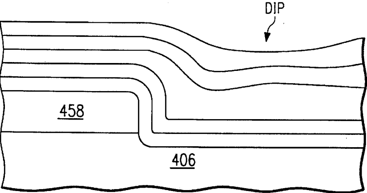
FIG. 4l (CROSS SECTION)
