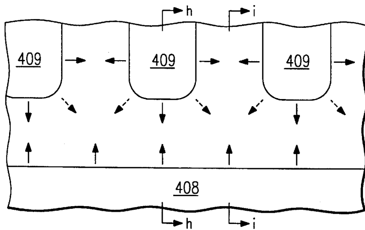
FIG. 4g (PLAN VIEW)
