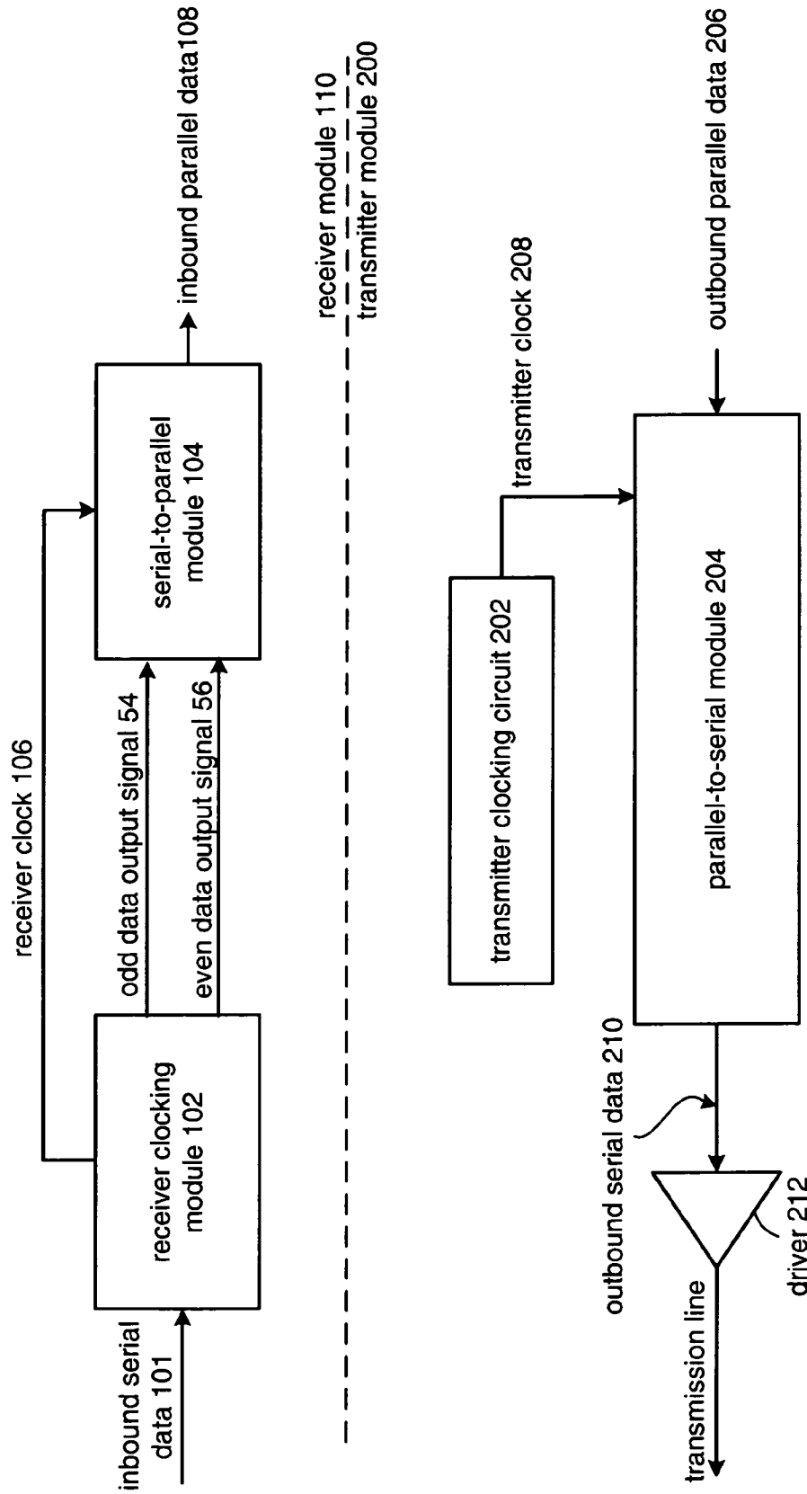
FIG. 9 transceiver 100
