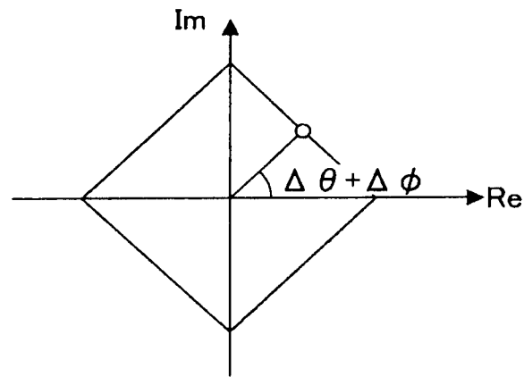
(c) WHEN PERIODIC SIGNAL IS RECTANGULAR WAVE
