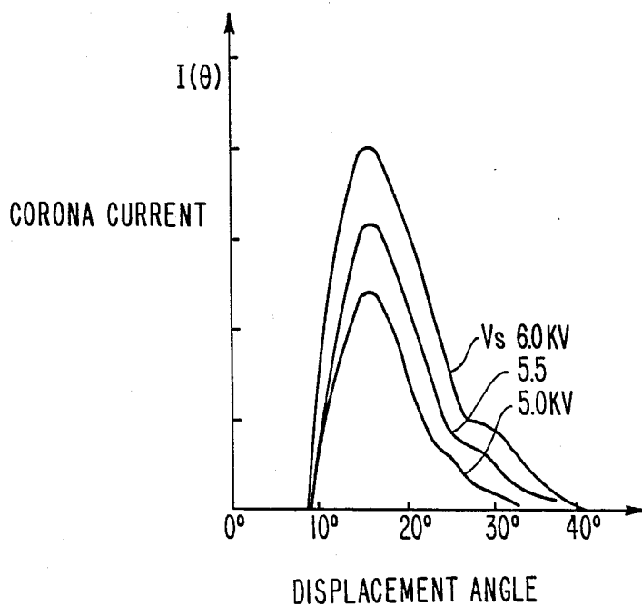
FIG. 7 (PRIOR ART)
