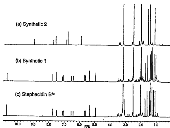
Figure 2. ^1\text{H} NMR spectra at 23 °C (500 MHz, 1:1 DMSO- d_6 - \text{CD}_3\text{CN} ) of (a) synthetic “avrainvillamide” (2), (b) synthetic stephacidin B (1), (c) stephacidin B from a fungal source
