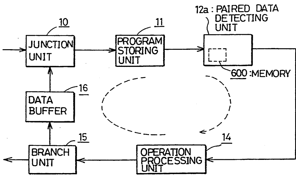
FIG.10 PRIOR ART
