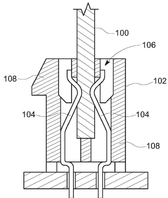
FIG. 1 (PRIOR ART)
