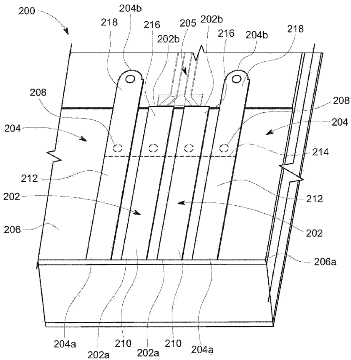
FIG. 2 (PRIOR ART)
