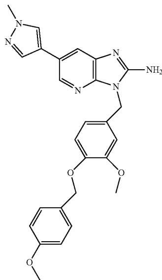
Formula (I): 3-(3-methoxy-4-((4-methoxybenzyl)oxy)benzyl)-6-(1-methyl-1H-pyrazol-4-yl)-3H-imidazo[4,5-b]pyridin-2-amine (GZ389988)
