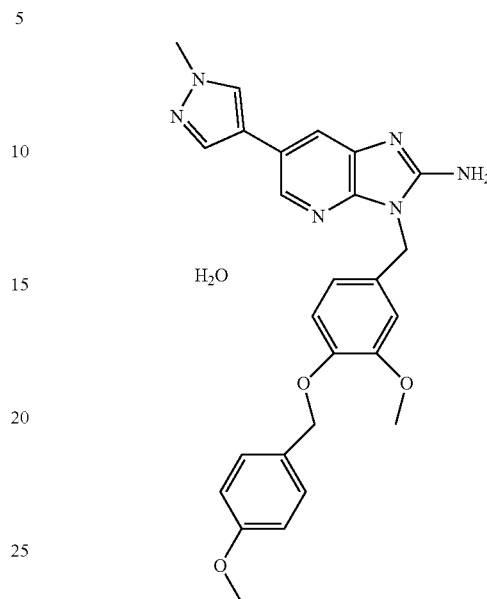
Formula (II): Monohydrate Form of 3-(3-methoxy-4-((4-methoxybenzyl)oxy)benzyl)-6-(1-methyl-1H-pyrazol-4-yl)-3H-imidazo[4,5-b]pyridin-2-amine (GZ389988A)
