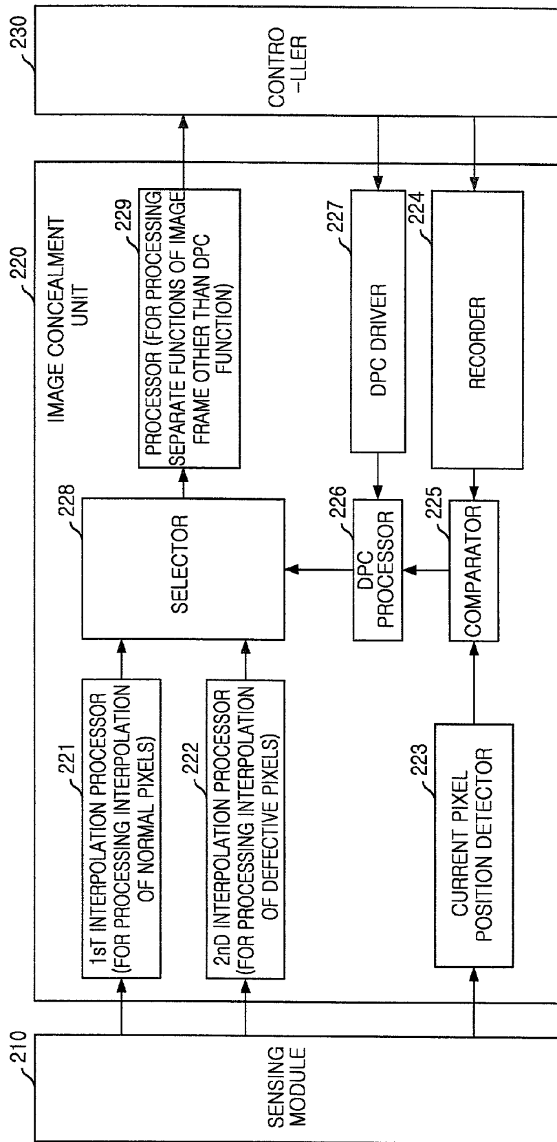
FIG. 2C (PRIOR ART)
