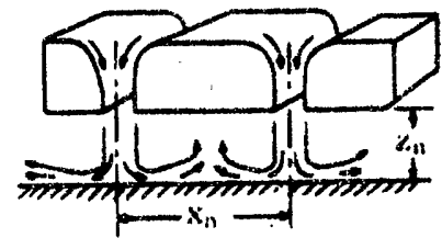
Fig. 2 Array of parallel slot jets with nozzle-shape slots.
