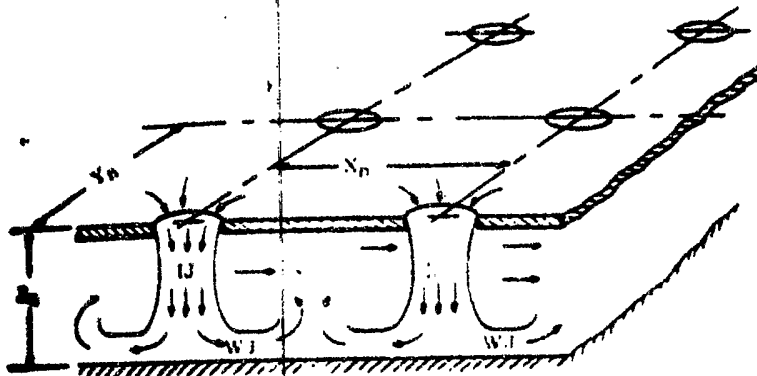
Fig. 1 Array of round jets in thin plate.
