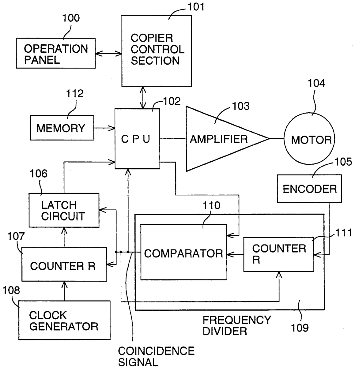
SPEED CONTROL CIRCUIT OF MOTOR
