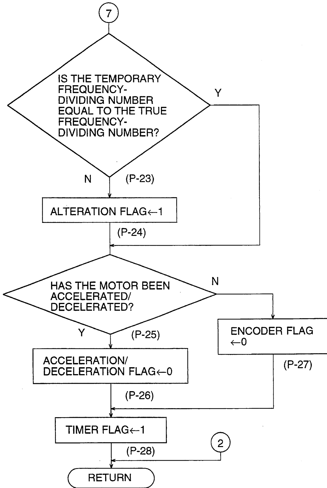
FIG. 5 TIMER INTERRUPTION PROCESSING(3)
