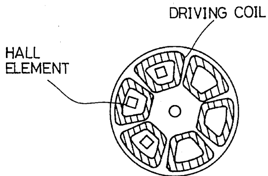
STATOR DRIVING COIL
