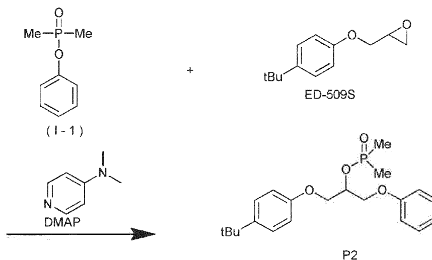
[Chem. 13]
