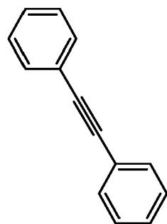
Diphenylacetylene
