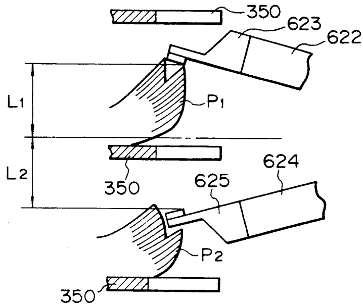
Fig. 1 PRIOR ART
