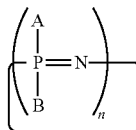
[Chemical Formula-5]
