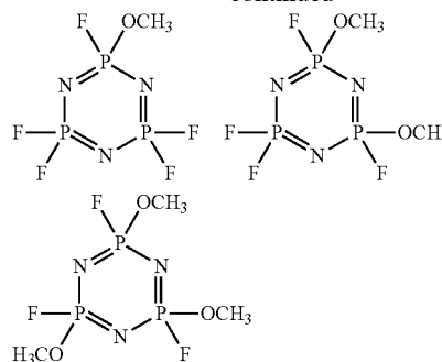
(cyclotriphosphazenes having methyl group(s) through oxygen)
