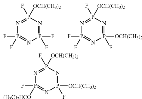
(cyclotriphosphazenes having isopropyl group(s) through oxygen)
