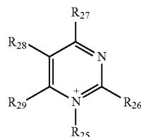
[Chemical Formula-29]
