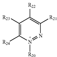
[Chemical Formula-27]
