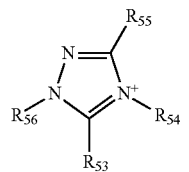
[Chemical Formula-34]
