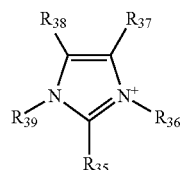
[Chemical Formula-31]
