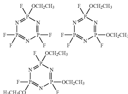
(cyclotriphosphazenes having ethyl group(s) through oxygen)
