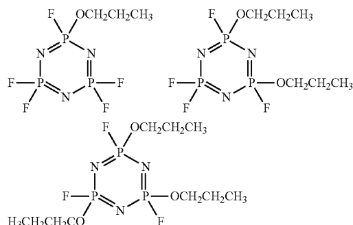
(cyclotriphosphazenes having propyl group(s) through oxygen)
