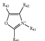
[Chemical Formula-32]
