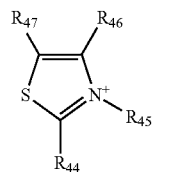
[Chemical Formula-33]
