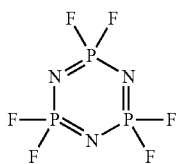
(cyclotriphosphazene wholly substituted with fluorine atoms)
