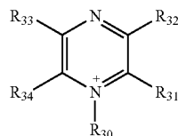
[Chemical Formula-30]
