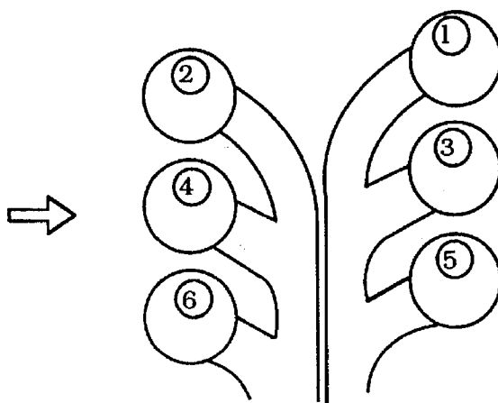
6- cylinder operation
