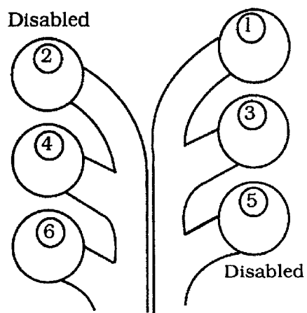
4- cylinder operation
