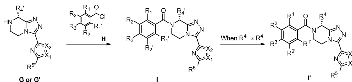
Scheme 16: Acylation.
