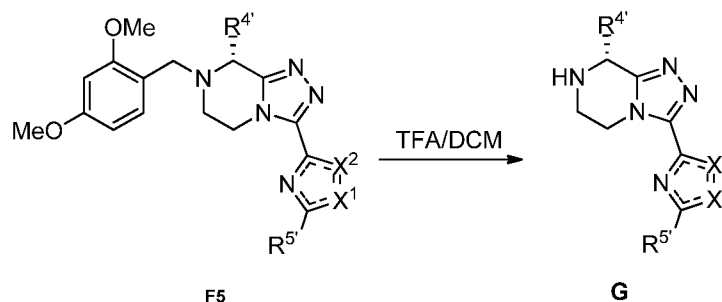
Scheme 14: DMB deprotection.
