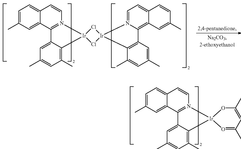
Compound 24
