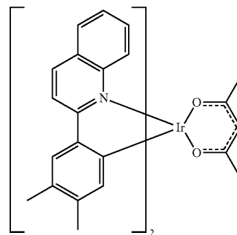
Compound 13
