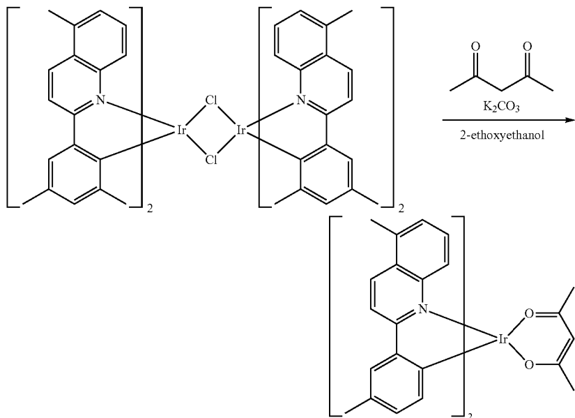
Compound 15
