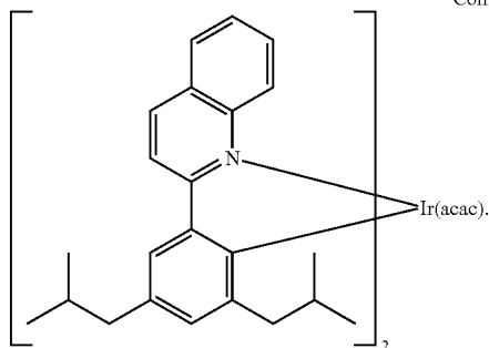
Compound 23
