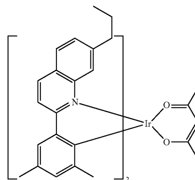
Compound 16
