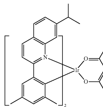
Compound 17
