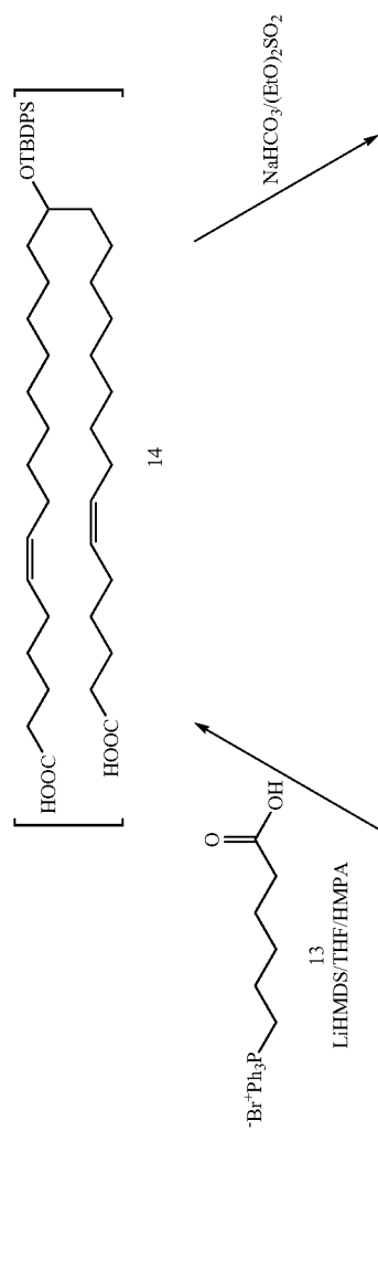
Scheme 2
