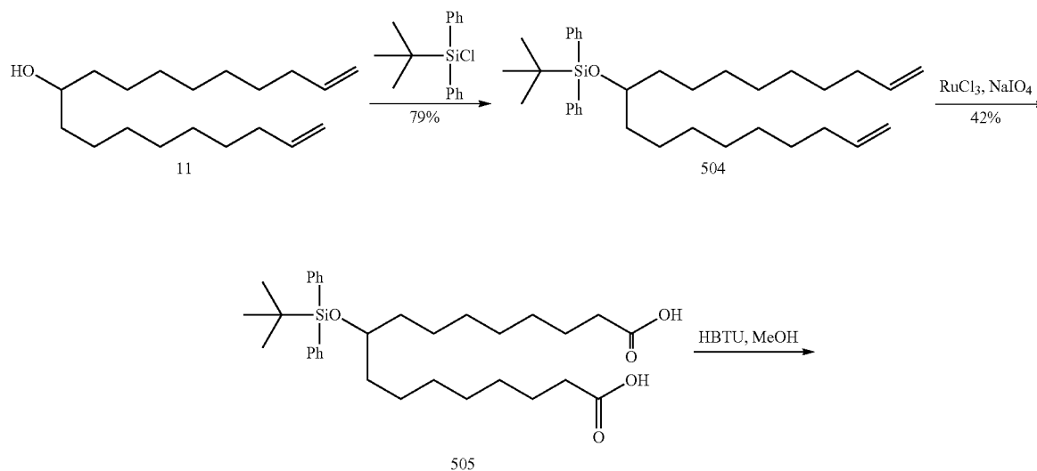
Scheme 25
