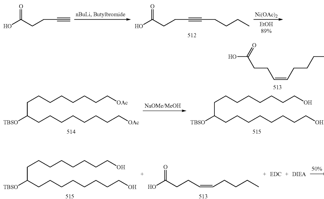
Scheme 26
