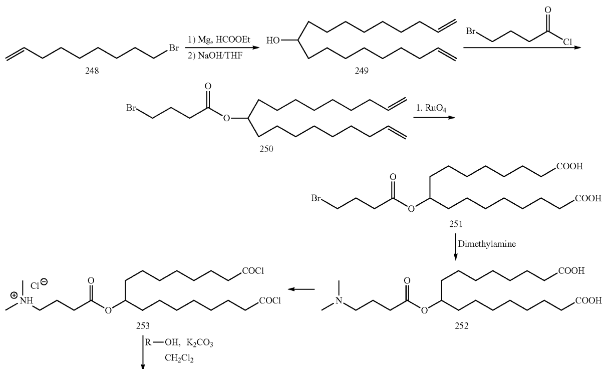
Scheme 18
