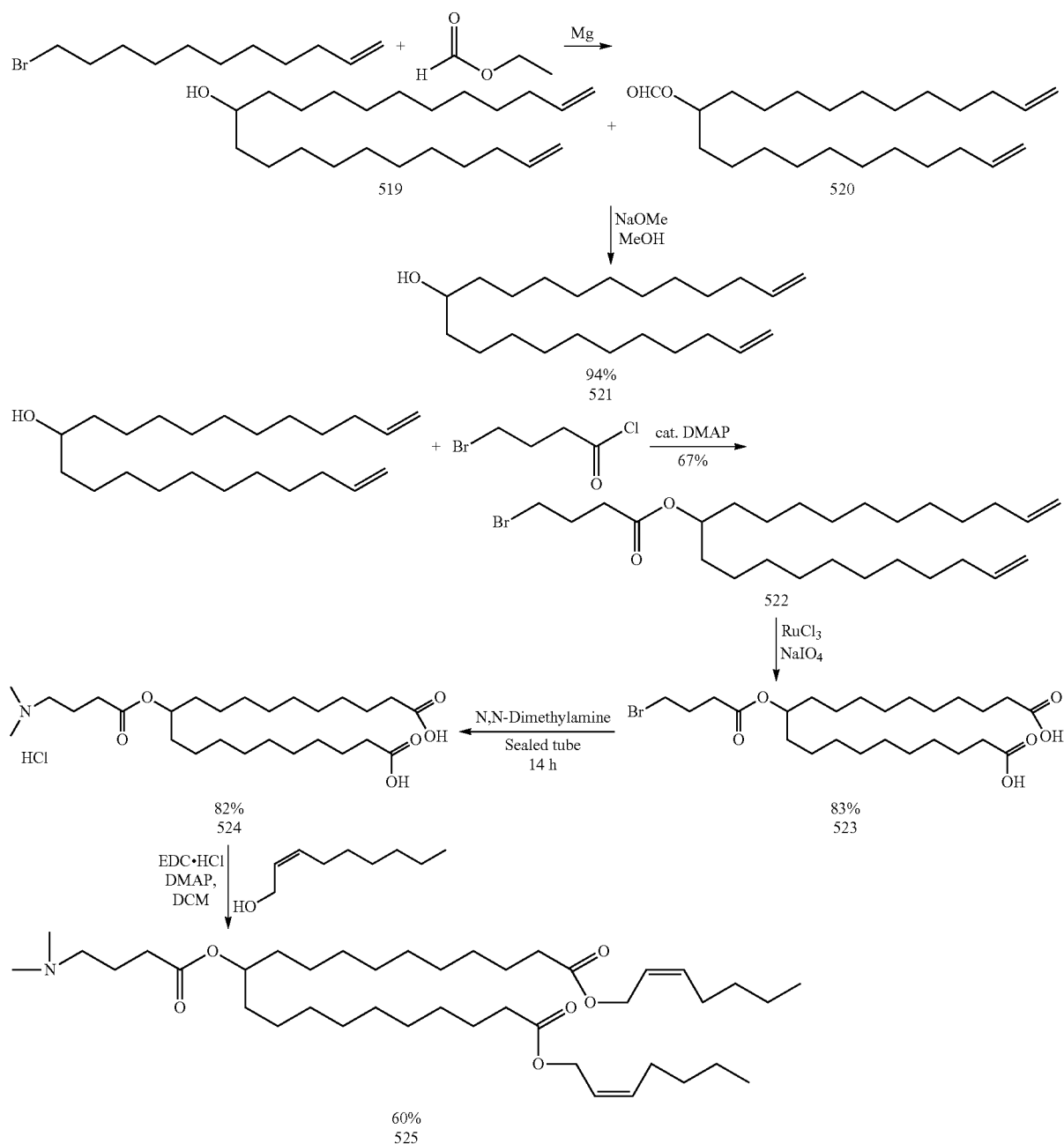
Scheme 27
