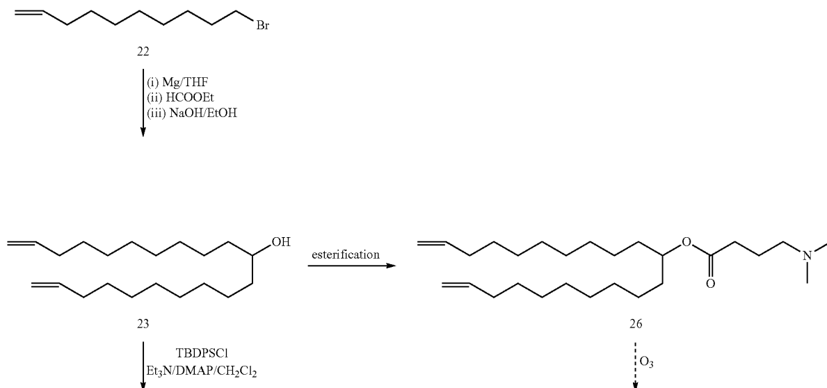
Scheme 3
