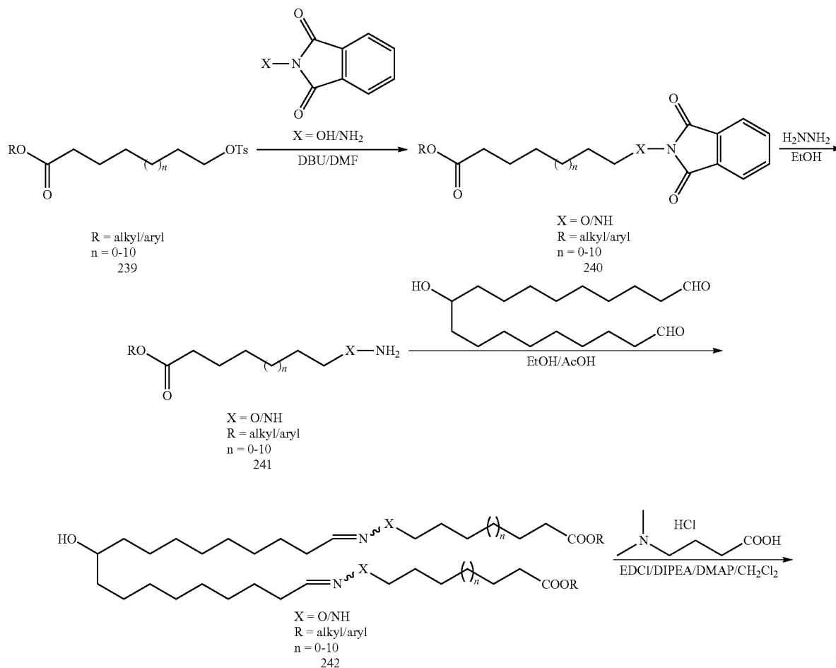
Scheme 29
