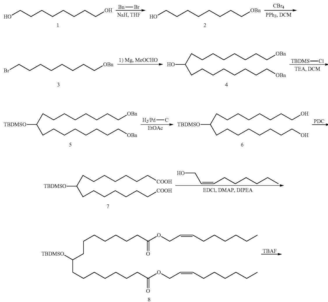
Scheme 20
