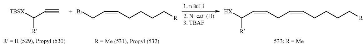
Scheme 28:
