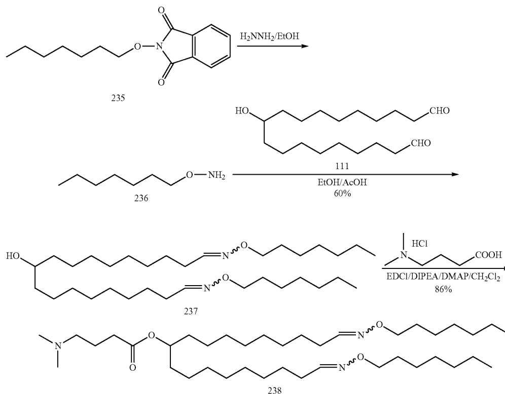
Scheme 16
