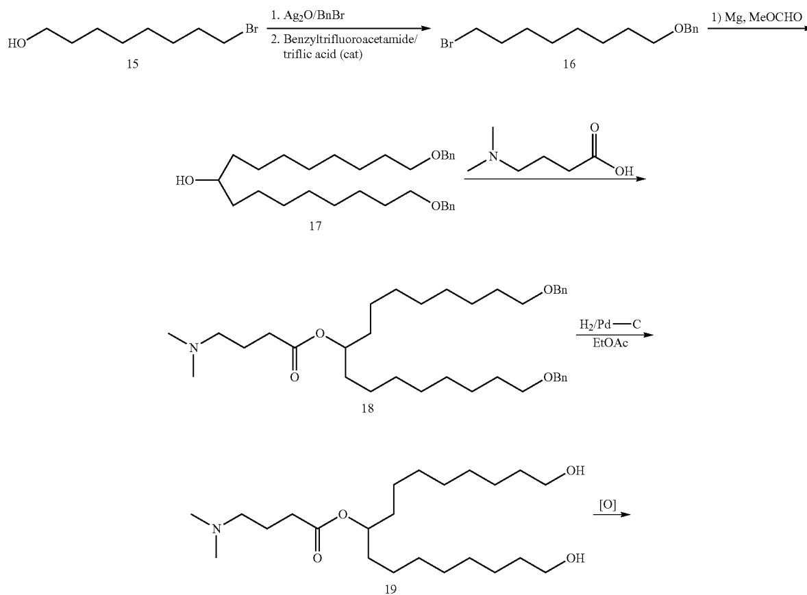
Scheme 19
