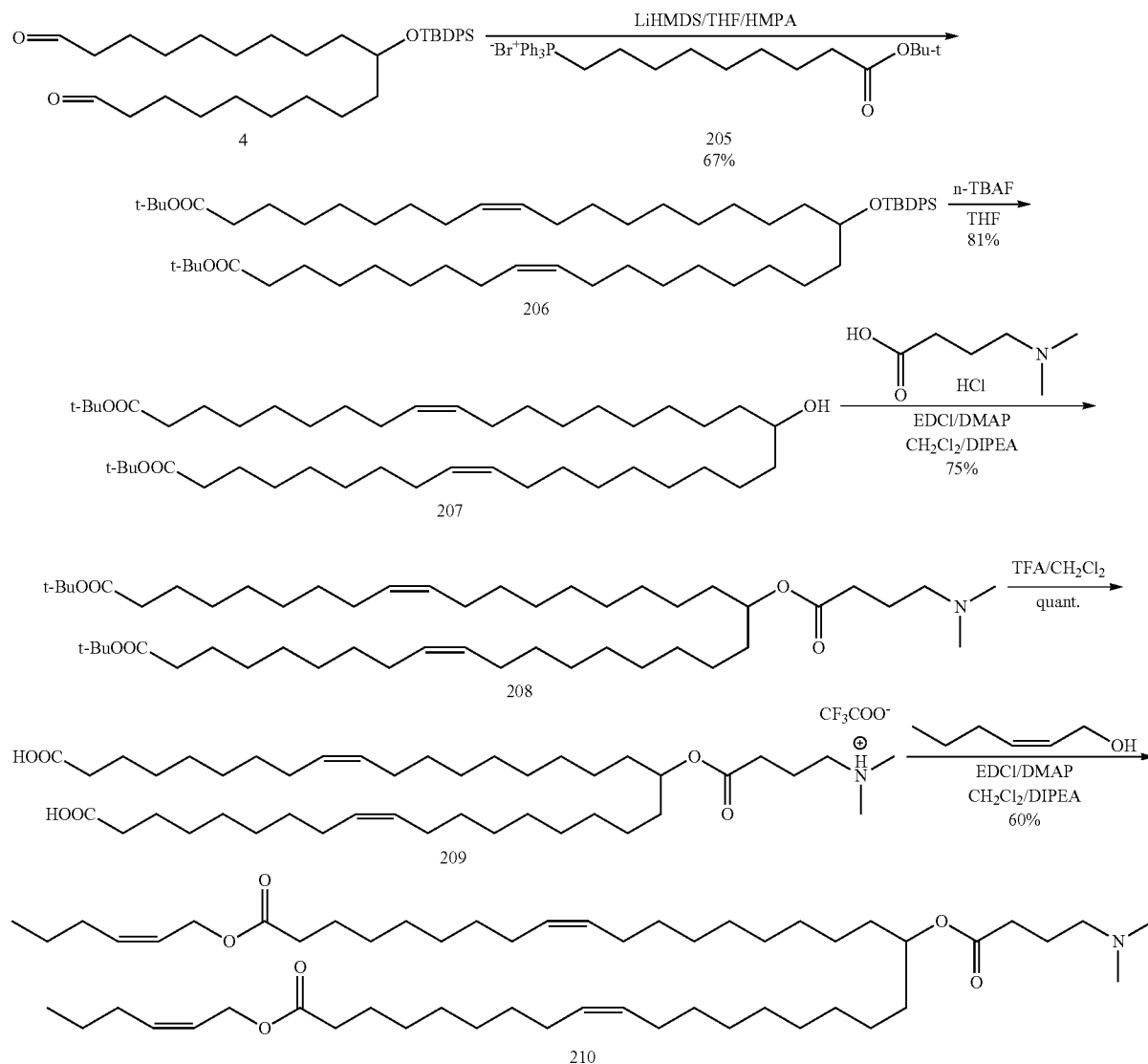
Scheme 10
