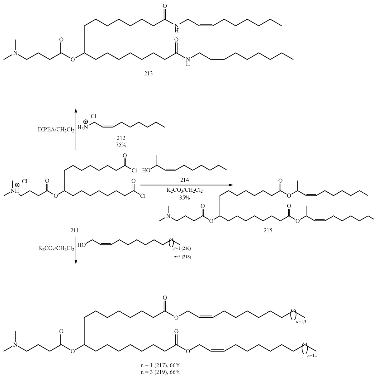
Scheme 11
