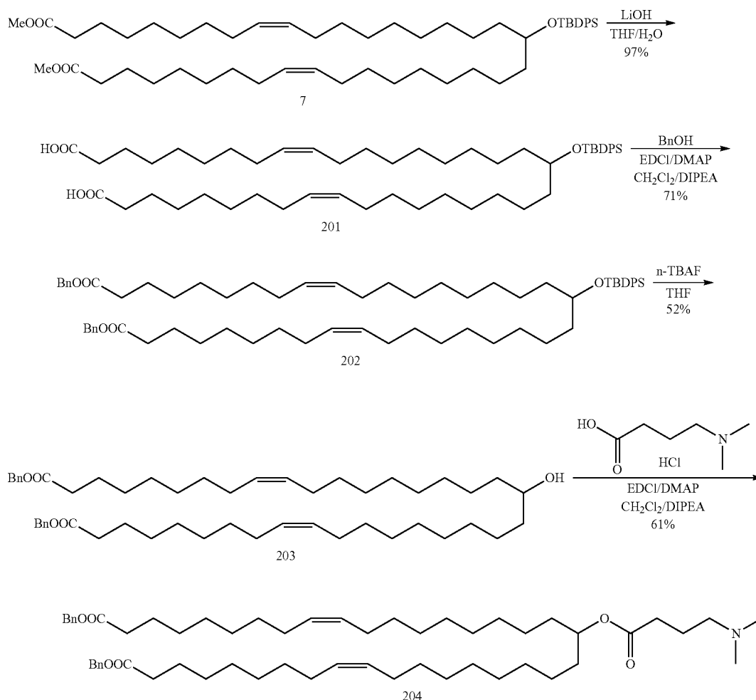
Scheme 9
