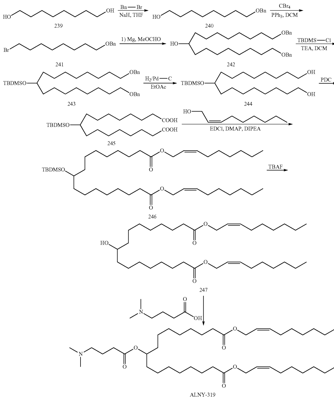
Scheme 17:
