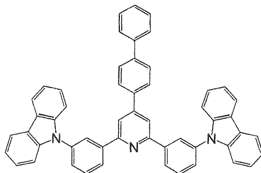
Compound C1
