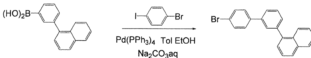
Compound 6
