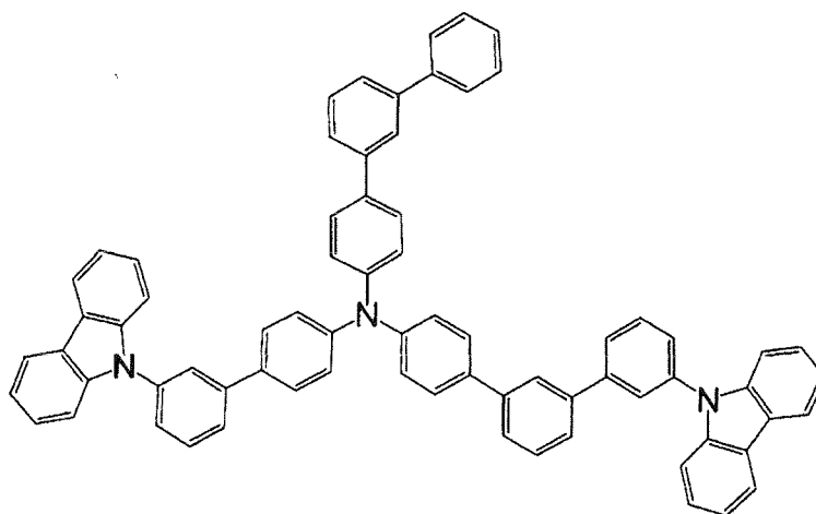
Compound I
