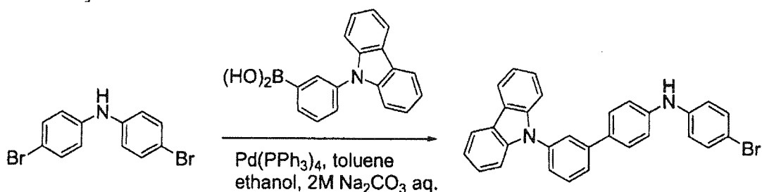
Compound 2
