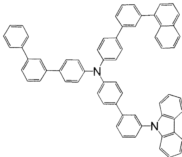
Compound II
