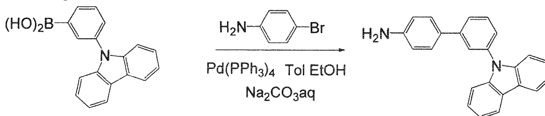
Compound 8
