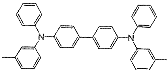
[Chem. 4]
