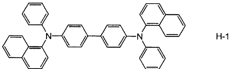
[Chem. 1]
