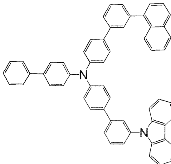
Compound III
