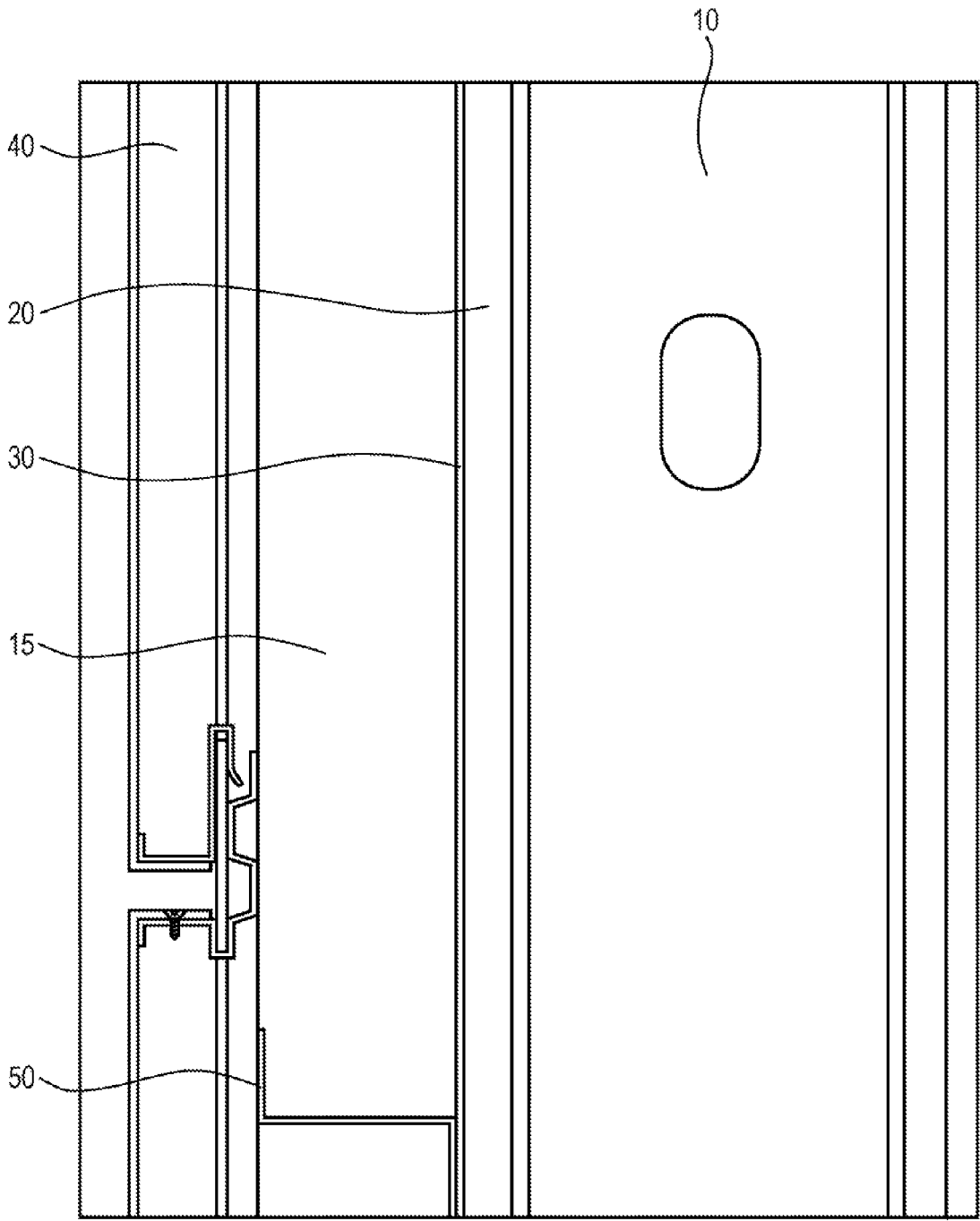
FIG. 2 (PRIOR ART)
