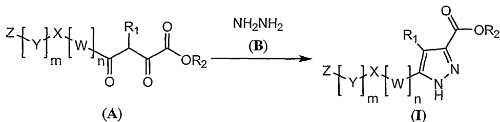
Reaction Scheme (1)
