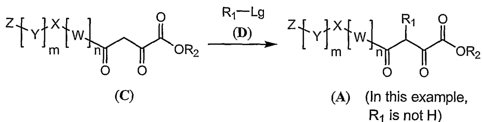
Reaction Scheme (2)
