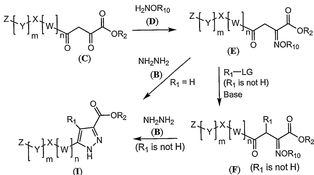
Reaction Scheme (3)
