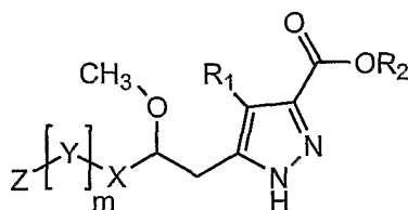
(In)
