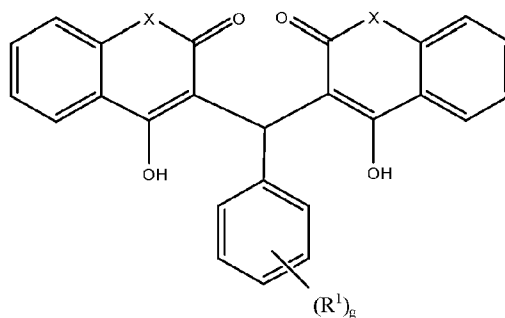
Formula III
