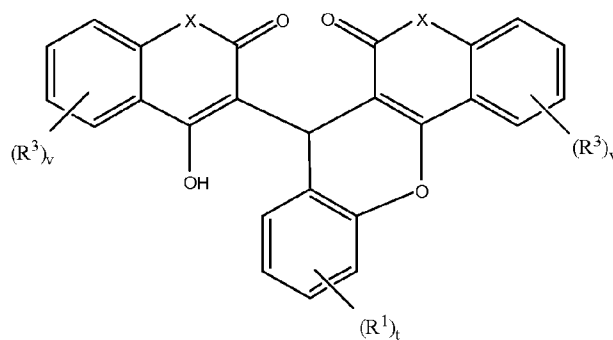
Formula XIV
