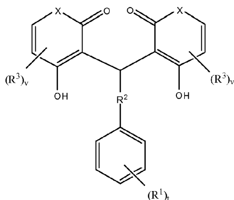
Formula XX
