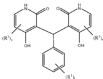
Formula XXV
