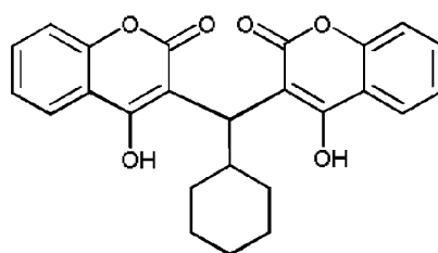
Compound 733
