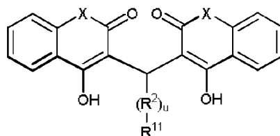
Formula A
