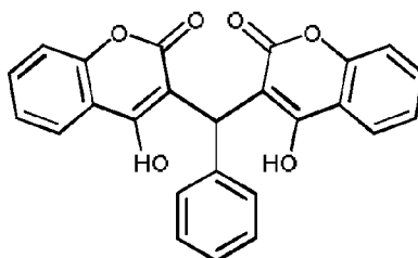
Compound 739
