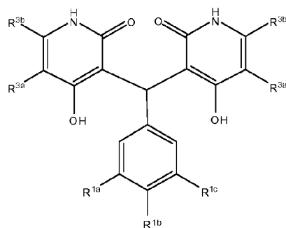
Formula XXVa
