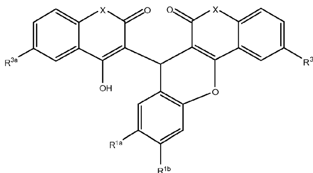
Formula XVa
