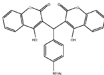
Compound 732
