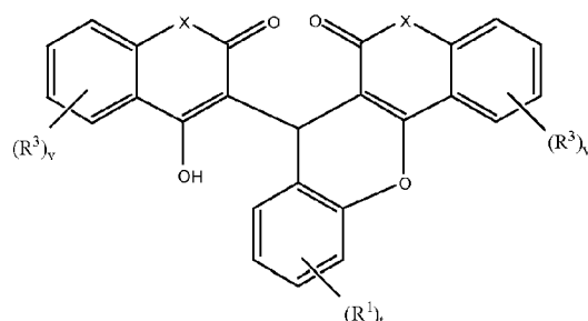
Formula XIV
