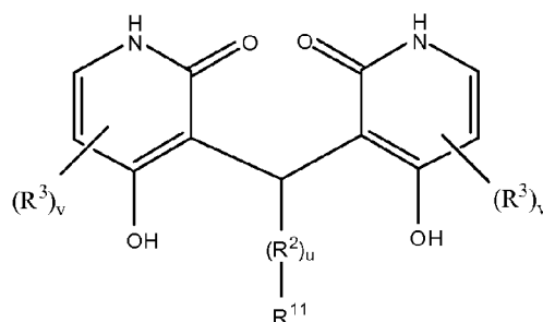
Formula F
