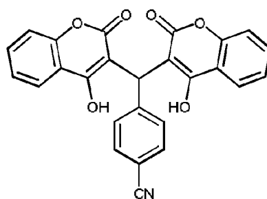
Compound 736
