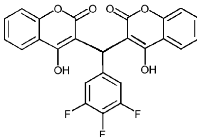
Compound 37
