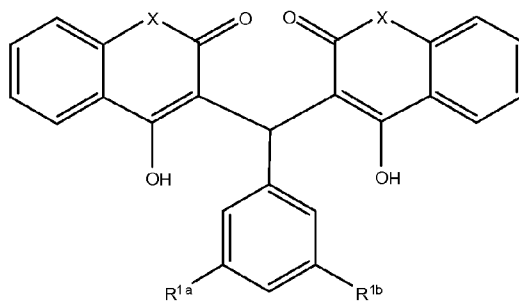
Formula IVa
