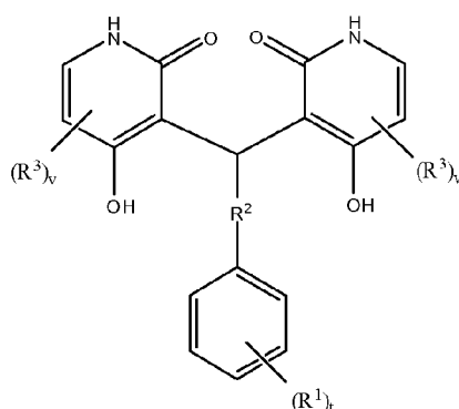
Formula XXIV
