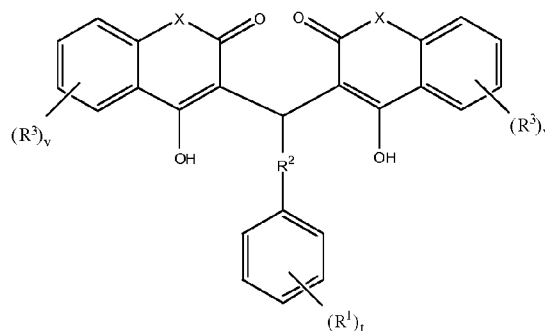
Formula VII
