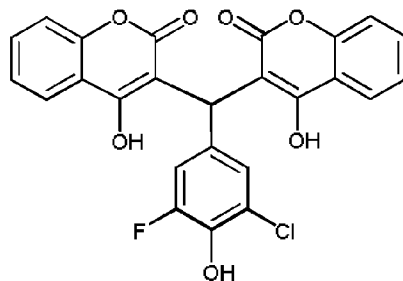
Compound 42
