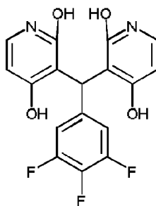
Compound 738
