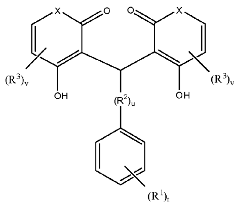
Formula E
