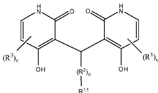
Formula F
