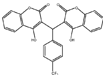
Compound 728
