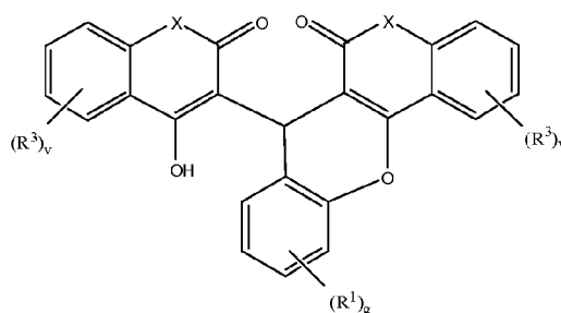
Formula XV
