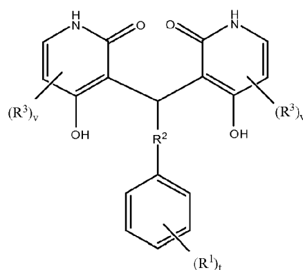
Formula XXIV
