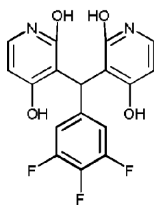
Compound 738
