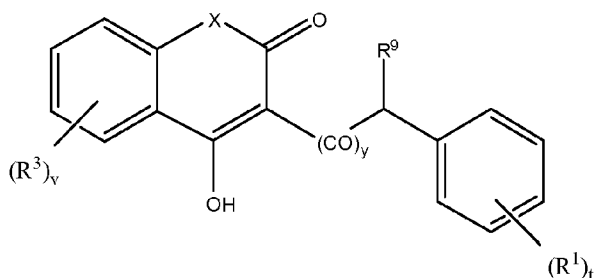
Formula D
