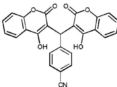
Compound 736
