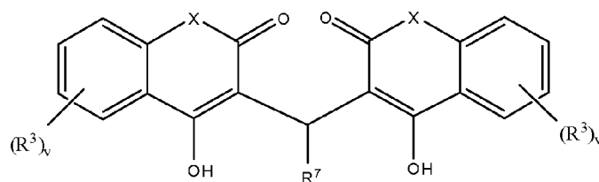
Formula XIII
