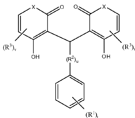
Formula E
