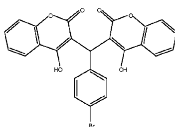
Compound 730
