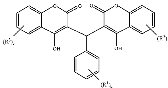
Formula X
