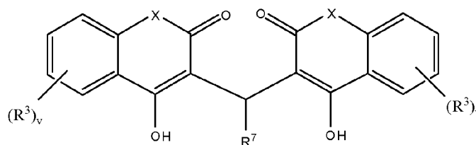
Formula XIII
