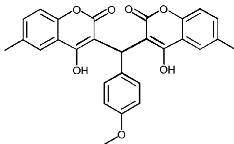
Compound 737
