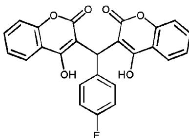
Compound 735
