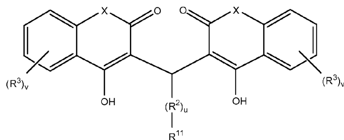
Formula B
