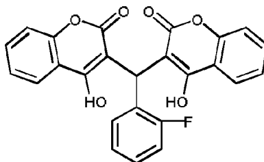
Compound 734
