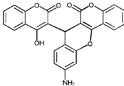
Compound 732
