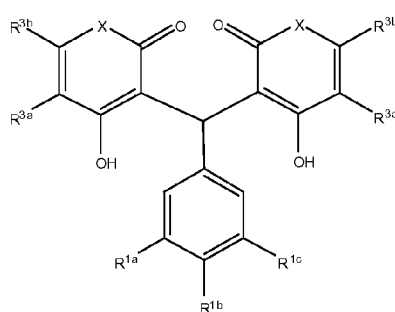
Formula XXIIa
