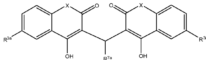
Formula XIIIa
