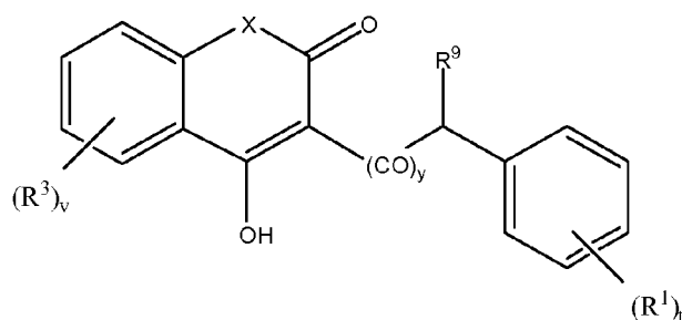
Formula D
