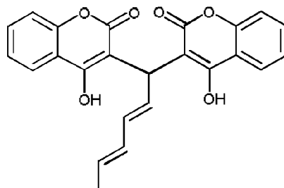
Compound 257
