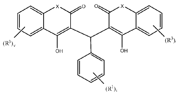
Formula VIII
