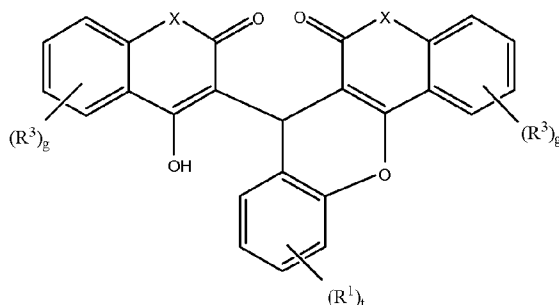
Formula XVI
