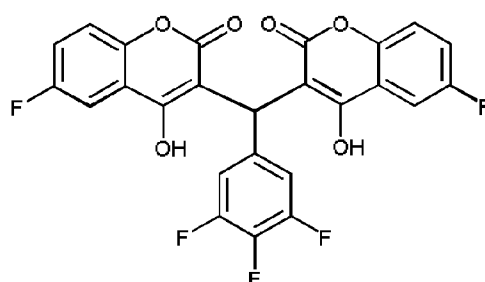
Compound 203
