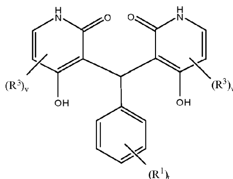
Formula XXV
