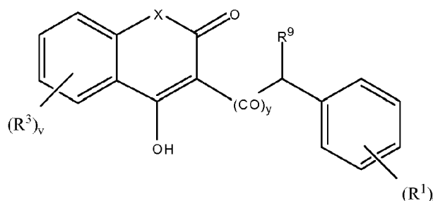
Formula D
