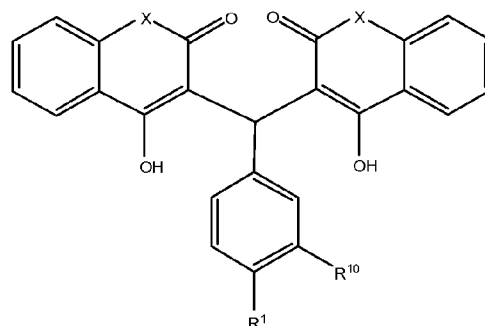
Formula VI
