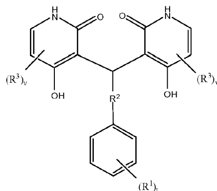
Formula XXIV
