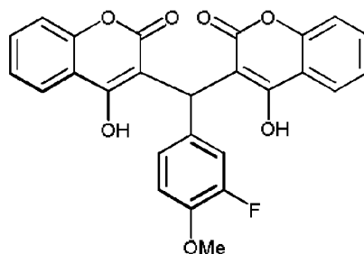
Compound 77
