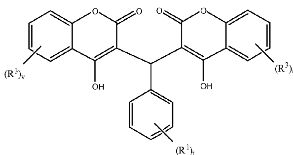
Formula IX
