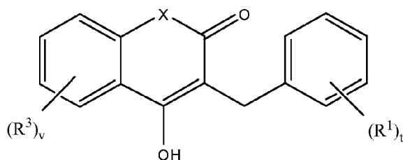
Formula XVII
