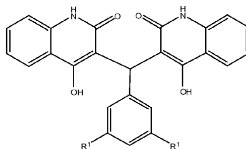
Formula V
