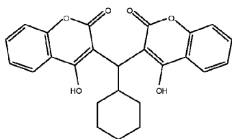
Compound 733
