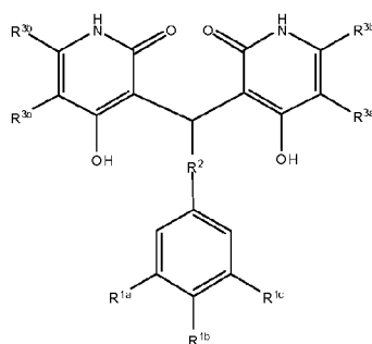
Formula XXIVa
