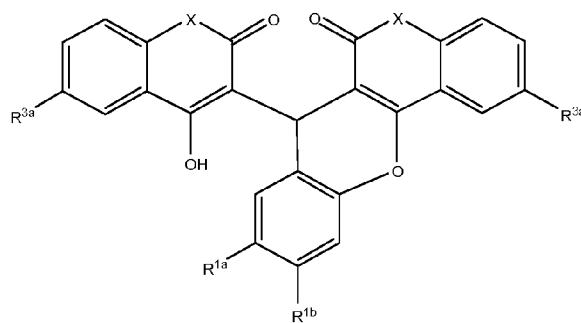
Formula XIVa
