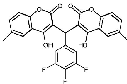
Compound 197
