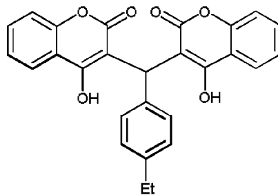
Compound 210
