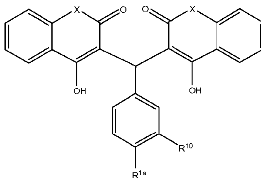
Formula VIa
