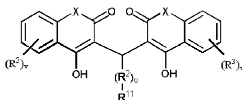
Formula B
