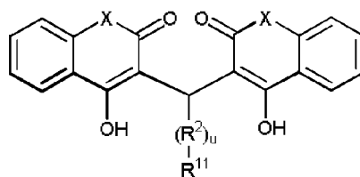
Formula A
