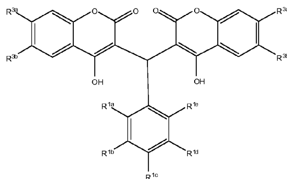
Formula Xa
