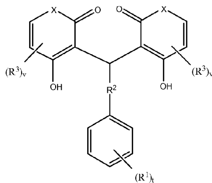
Formula XX
