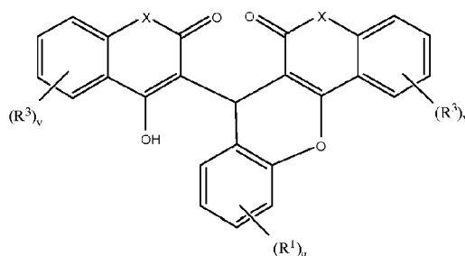
Formula XV
