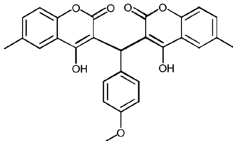
Compound 737
