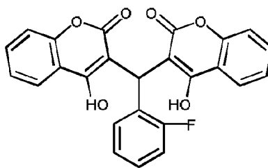
Compound 734,
