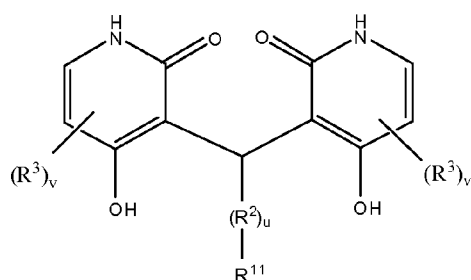
Formula F
