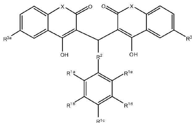
Formula VIIa
