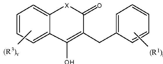
Formula XVII
