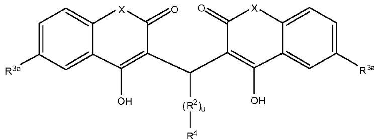
Formula XIa
