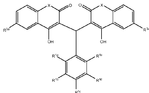
Formula VIIIa
