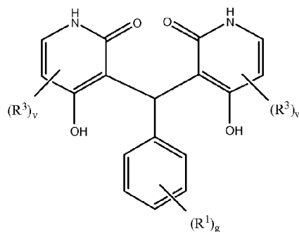
Formula XXVI
