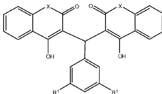
Formula IV
