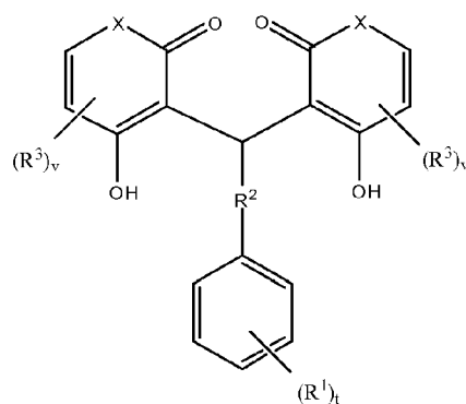
Formula XX
