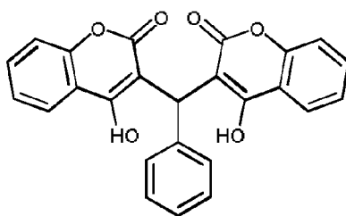
Compound 739
