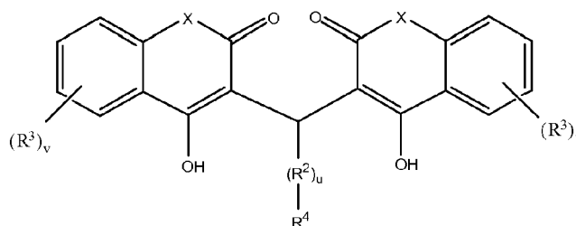
Formula XI
