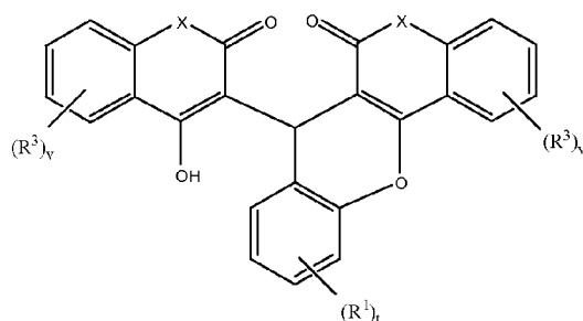
Formula XIV
