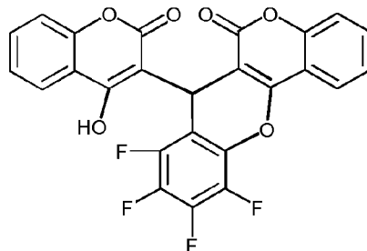
Compound 423
