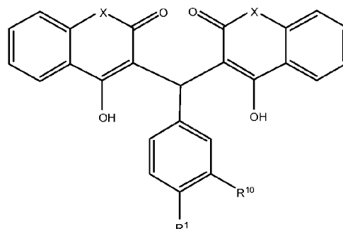
Formula VI
