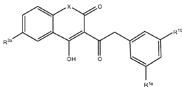
Formula XIXa
