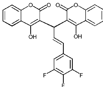
Compound 1
