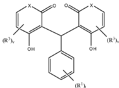
Formula XXI
