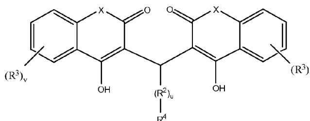
Formula XI
