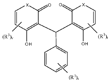
Formula XXI
