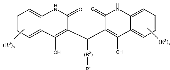
Formula XII
