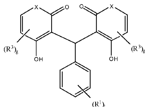
Formula XXIII
