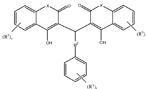
Formula VII
