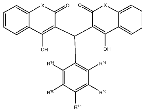
Formula IIIa
