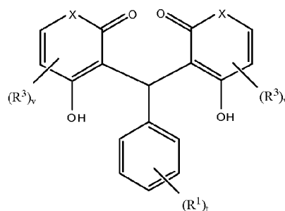
Formula XXI
