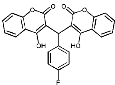
Compound 735
