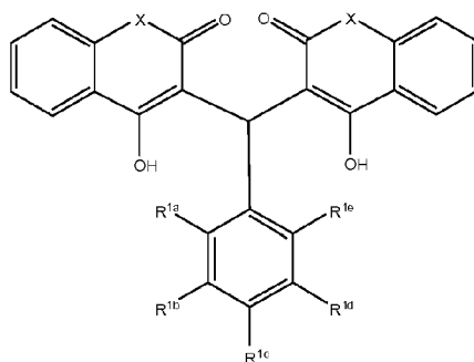
Formula IIa
