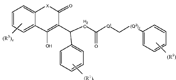
Formula XVIII
