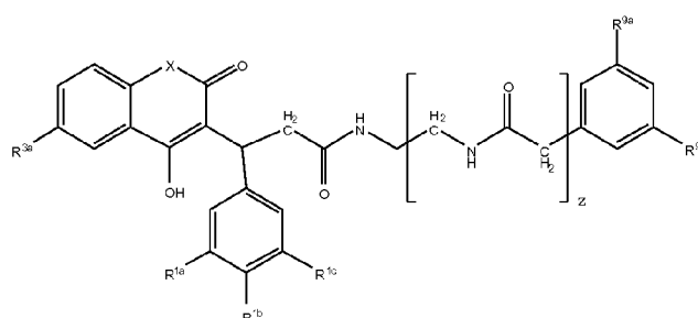
Formula XVIIIa
