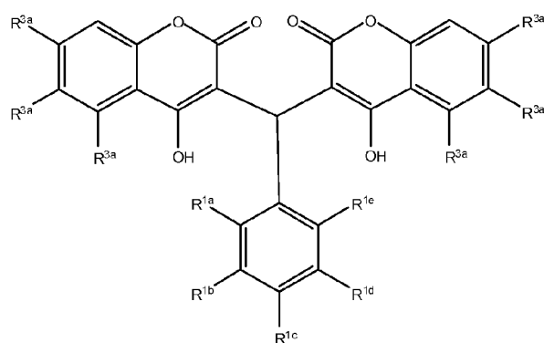
Formula IXa
