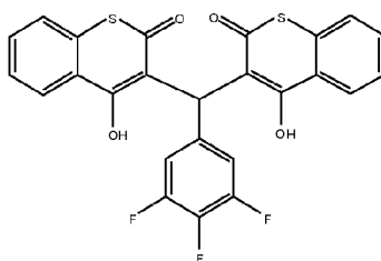
Compound 53
