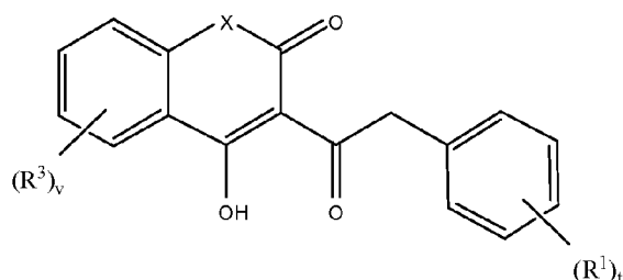
Formula XIX
