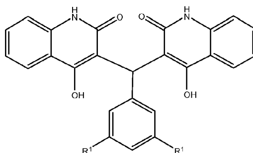
Formula V
