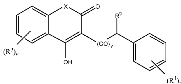
Formula D
