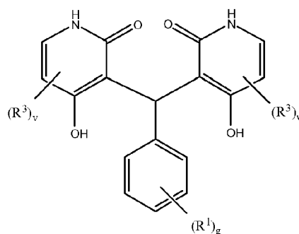
Formula XXVI
