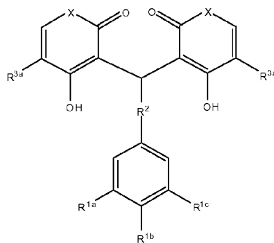
Formula XXa
