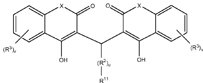
Formula B
