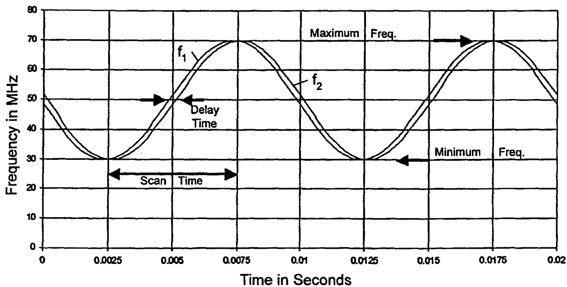
Frequencies of Drive Waveforms vs. Time: Sinusoidal Ramp
