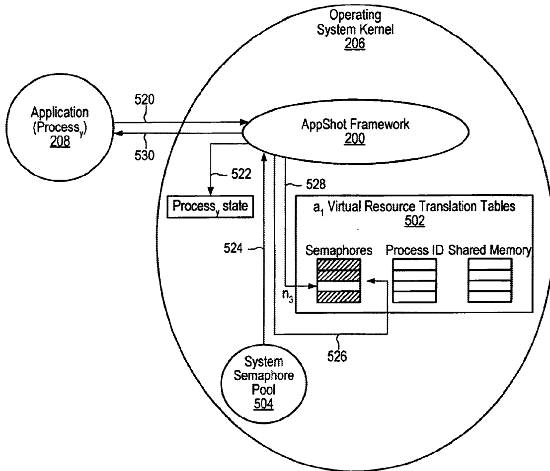
Allocation of a virtual resource (i.e. semaphore)
