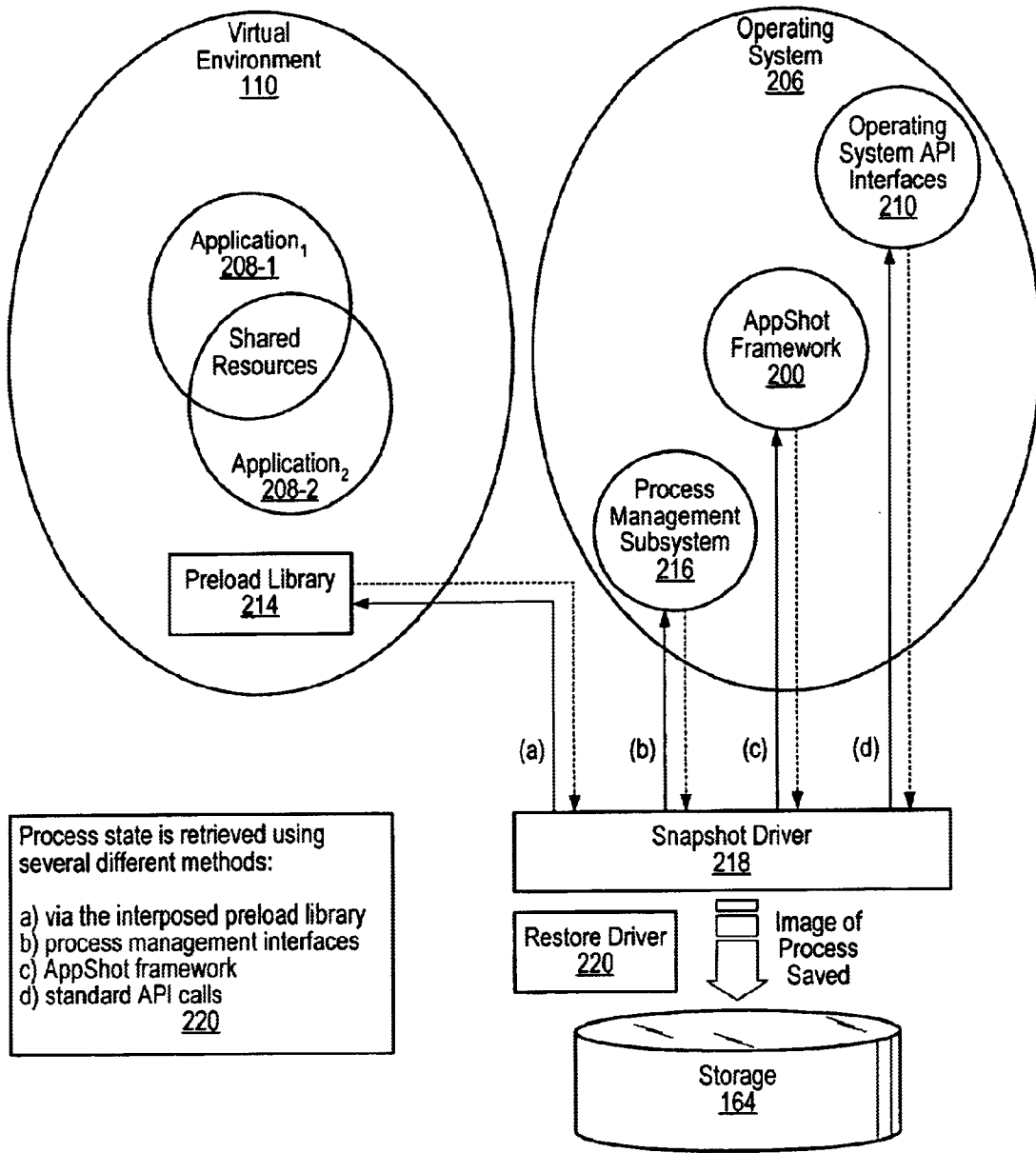
Capture of an application's run-time state.
