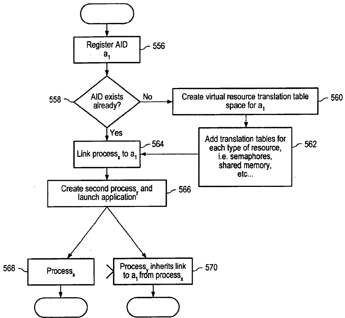
Flowchart describing creation of virtual translation tables
