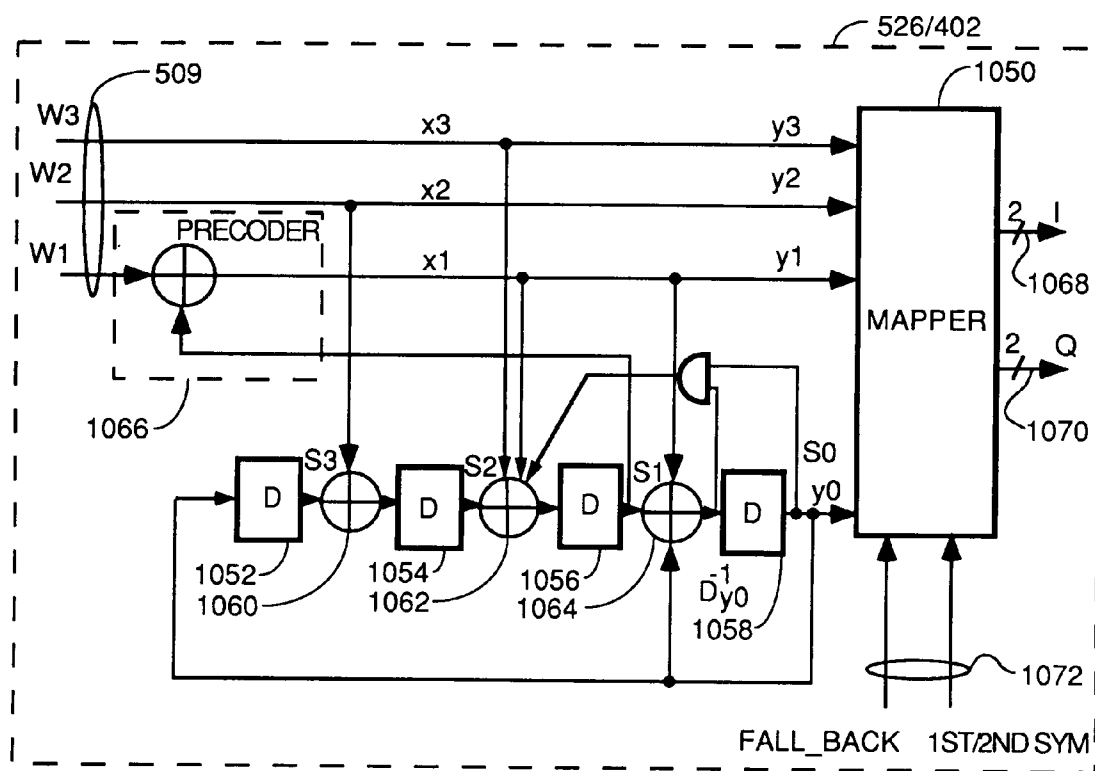
PREFERRED TRELLIS ENCODER
