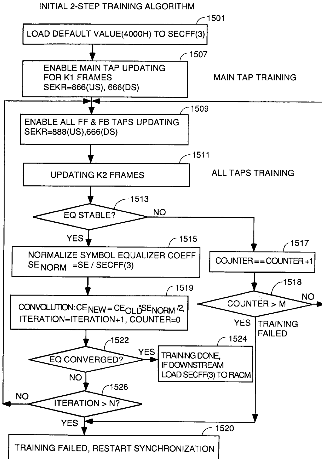
2-STEP INITIAL EQUALIZATION TRAINING
