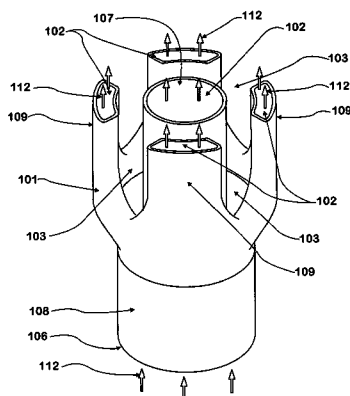
MIXING DEVICE WITH EXHAUST FLOW
