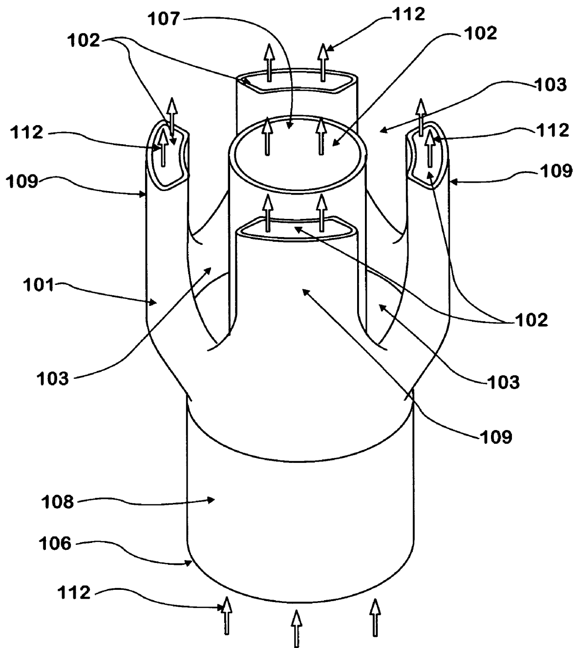
FIG. 1 MIXING DEVICE WITH EXHAUST FLOW
