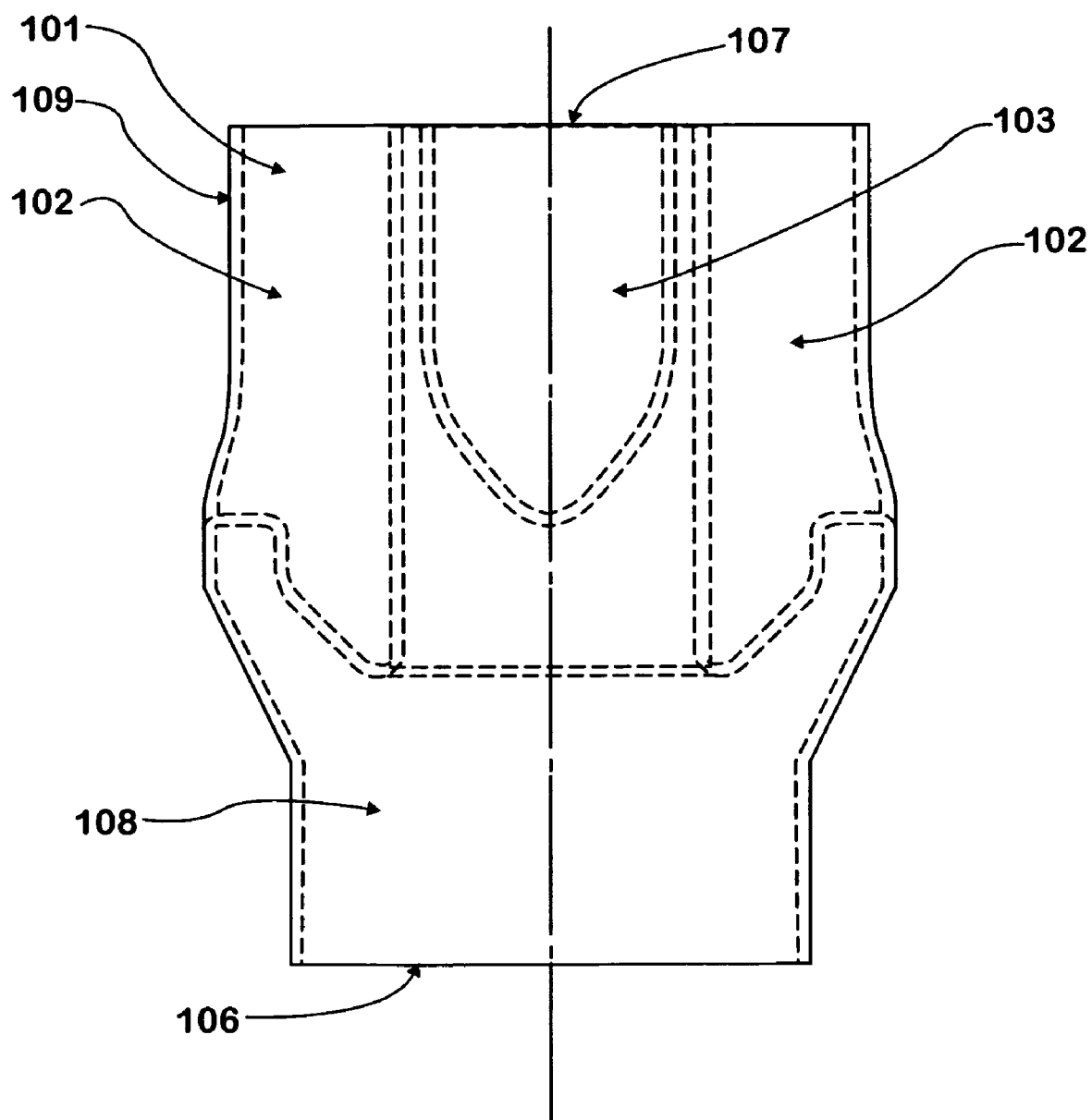
FIG. 5 MIXING DEVICE
