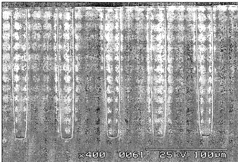
20um diameter ~ 150um deep
