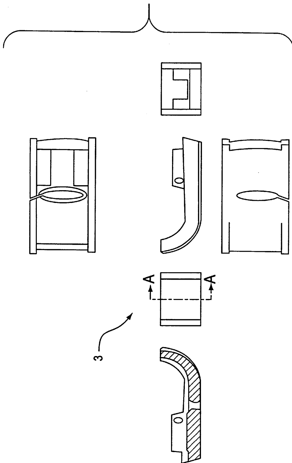
FIG. 2 (PRIOR ART)
