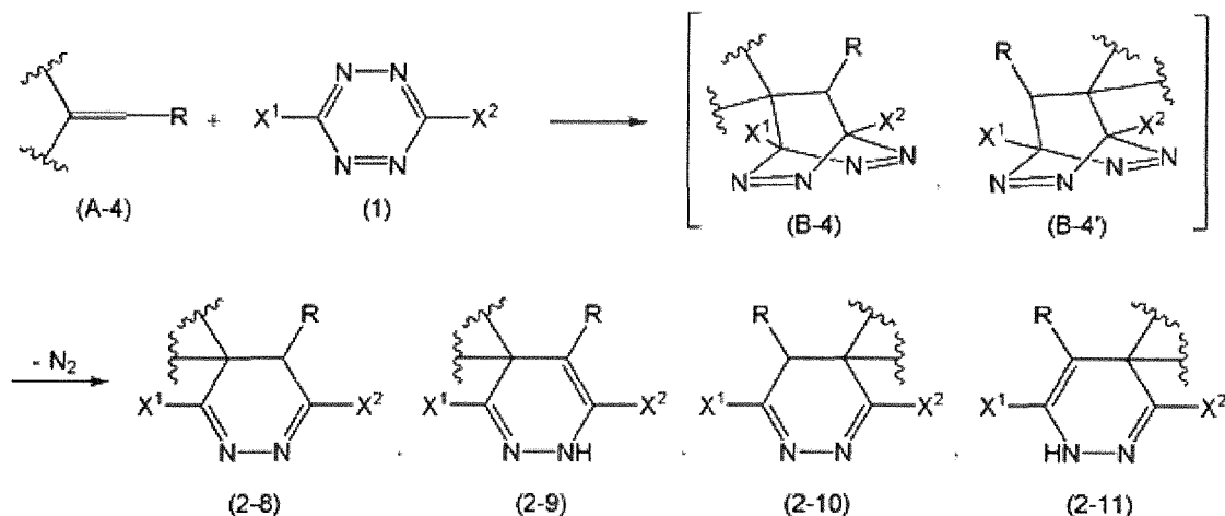
Reaction Scheme-4
