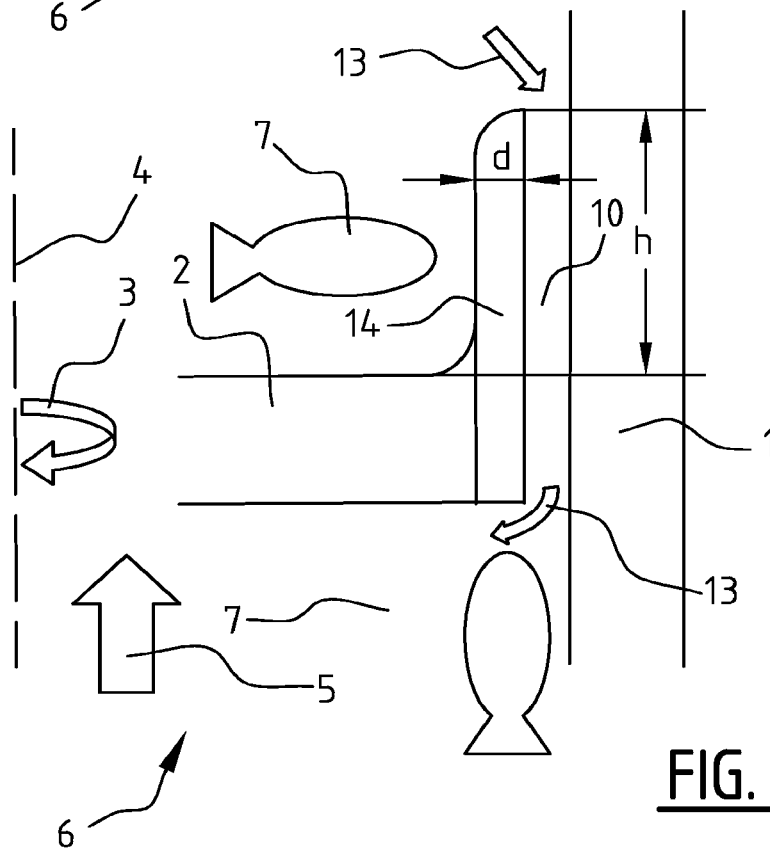
FIG. 1 - Prior Art
