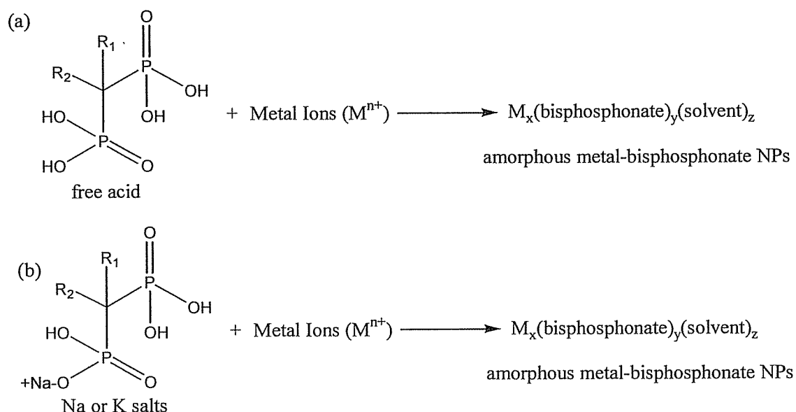
Scheme 3. Synthesis of Amorphous Metal-Bisphosphonate Nanoparticles.
