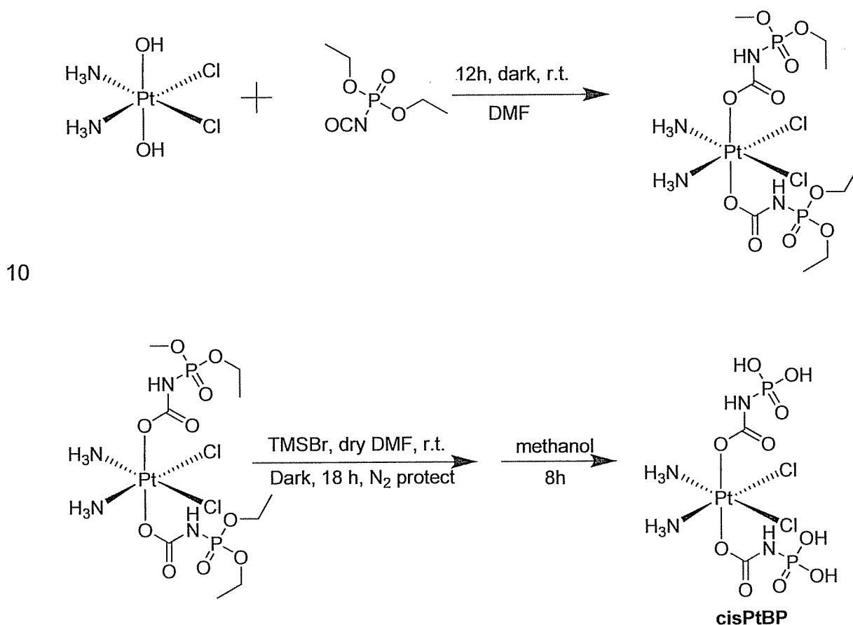
Scheme 4. Synthesis of Cisplatin Bisphosphonate Complex.
