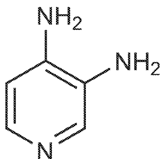
3,4-diaminopyridine
